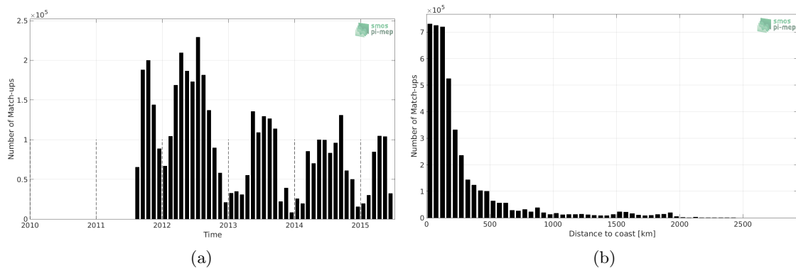
Figure 1: Number of match-ups between TSG-SAMOS and Aquarius-L3-OR-V5-7DAY-RUNNING-1DEG SSS as a function of time (a) and as function of the distance to coast (b) over the Global Ocean Pi-MEP region and for the full satellite product period.
