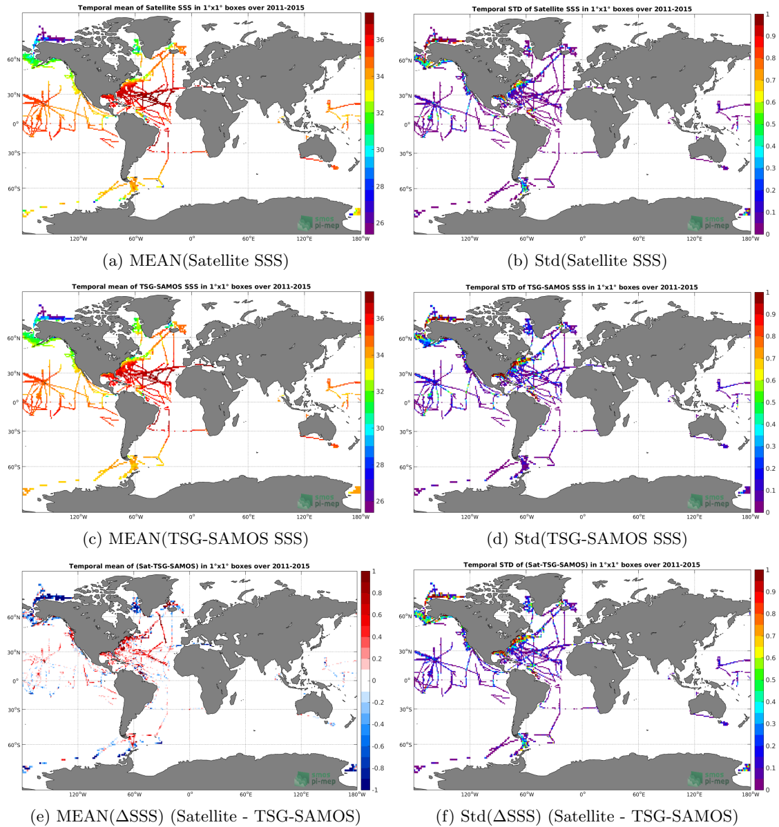
Figure 6: Temporal mean (left) and Std (right) of SSS from Aquarius-L3-OR-V5-7DAY-RUNNING-1DEG (top), TSG-SAMOS (middle), and of \Delta SSS (Satellite - TSG-SAMOS). Only match-up pairs are used to generate these maps.
