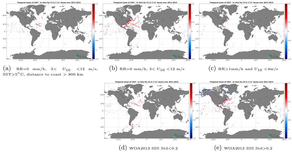
Figure 12: Temporal mean gridded over spatial boxes of size 1^\circ \times 1^\circ of \Delta SSS (Aquarius-L3-OR-V5-7DAY-RUNNING-1DEG - TSG-SAMOS) for 5 different subdatasets corresponding to:RR=0 mm/h, 3 < U_{10} < 12 m/s, SST >5^\circ C, distance to coast > 800 km (a), RR=0 mm/h, 3 < U_{10} < 12 m/s (b), RR >1 mm/h and U_{10} < 4 m/s (c), WOA2013 SSS Std <0.2 (d), WOA2013 SSS Std >0.2 (e).
