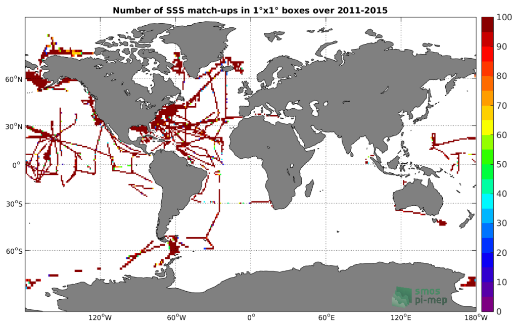
Figure 4: Number of SSS match-ups between TSG-SAMOS SSS and the Aquarius-L3-OR-V5-7DAY-RUNNING-1DEG SSS product for the Global Ocean Pi-MEP region over 1^\circ \times 1^\circ boxes and for the full satellite product period.
