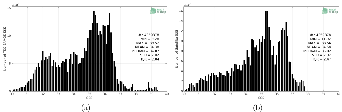
Figure 2: Histograms of SSS from TSG-SAMOS (a) and Aquarius-L3-OR-V5-7DAY-RUNNING-1DEG (b) considering all match-up pairs per bins of 0.1 over the Global Ocean Pi-MEP region and for the full satellite product period.
