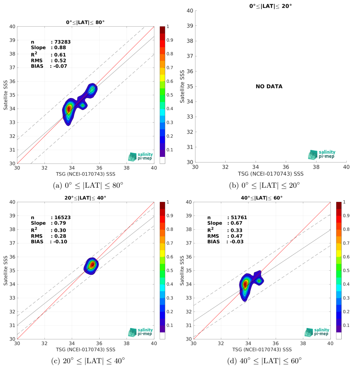
Figure 10: Contour maps of the concentration of Aquarius SSS L3 OR v5 - 7-Day running (NASA-GSFC) SSS (y-axis) versus TSG (NCEI-0170743) SSS (x-axis) at match-up pairs for different latitude bands. For each plot, the red line shows x=y . The black thin and dashed lines indicate a linear fit through the data cloud and the \pm 95\% confidence levels, respectively. The number match-up pairs n , the slope and R^2 coefficient of the linear fit, the root mean square (RMS) and the mean bias between satellite and in situ data are indicated for each latitude band in each plots.
