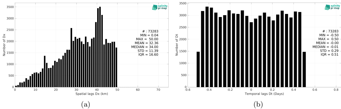
Figure 6: Histograms of the spatial (a) and temporal (b) lags between the location/time of the TSG (NCEI-0170743) measurement and the date of the corresponding Aquarius SSS L3 OR v5 - 7-Day running (NASA-GSFC) SSS pixel.
