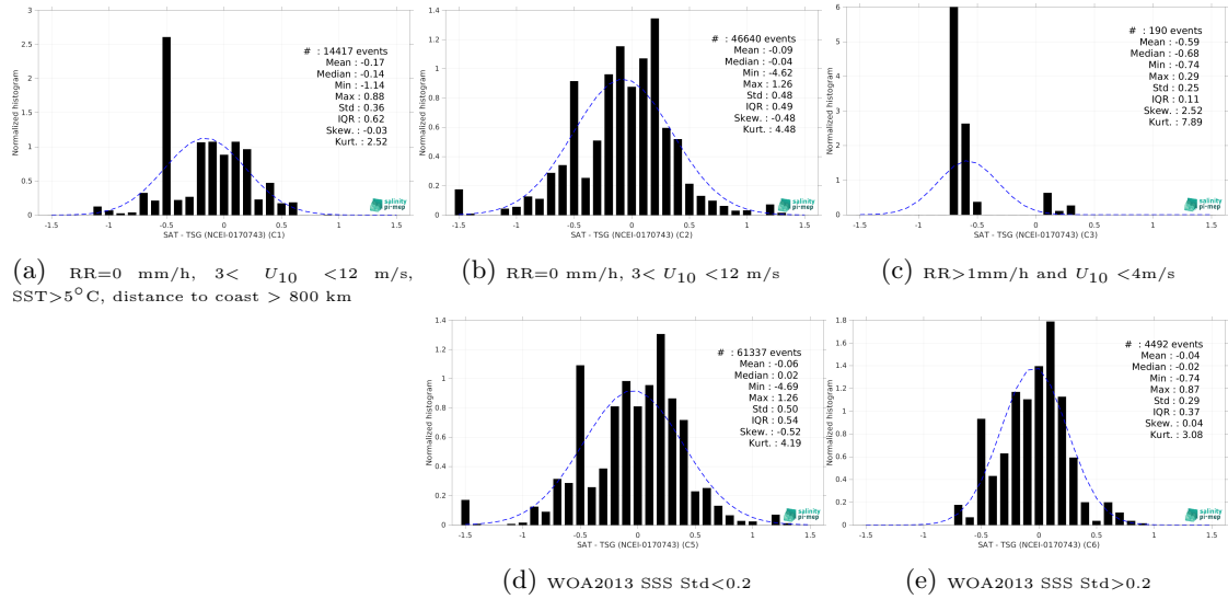
Figure 15: Normalized histogram of \Delta SSS (Aquarius SSS L3 OR v5 - 7-Day running (NASA-GSFC) - TSG (NCEI-0170743)) for 5 different subdatasets corresponding to: RR=0 mm/h, 3 < U_{10} < 12 m/s, SST > 5°C, distance to coast > 800 km (a), RR=0 mm/h, 3 < U_{10} < 12 m/s (b), RR > 1mm/h and U_{10} < 4 m/s (c), WOA2013 SSS Std < 0.2 (d), WOA2013 SSS Std > 0.2 (e).
