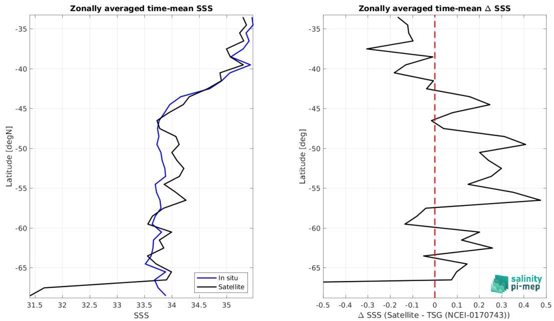
Figure 9: Left panel: Zonal mean SSS from Aquarius SSS L3 OR v5 - 7-Day running (NASA-GSFC) satellite product (black) and from TSG (NCEI-0170743) (blue). Right panel: Zonal mean of \Delta SSS (Satellite - TSG (NCEI-0170743)) for all the collected Pi-MEP match-up pairs estimated over the full satellite product period.
