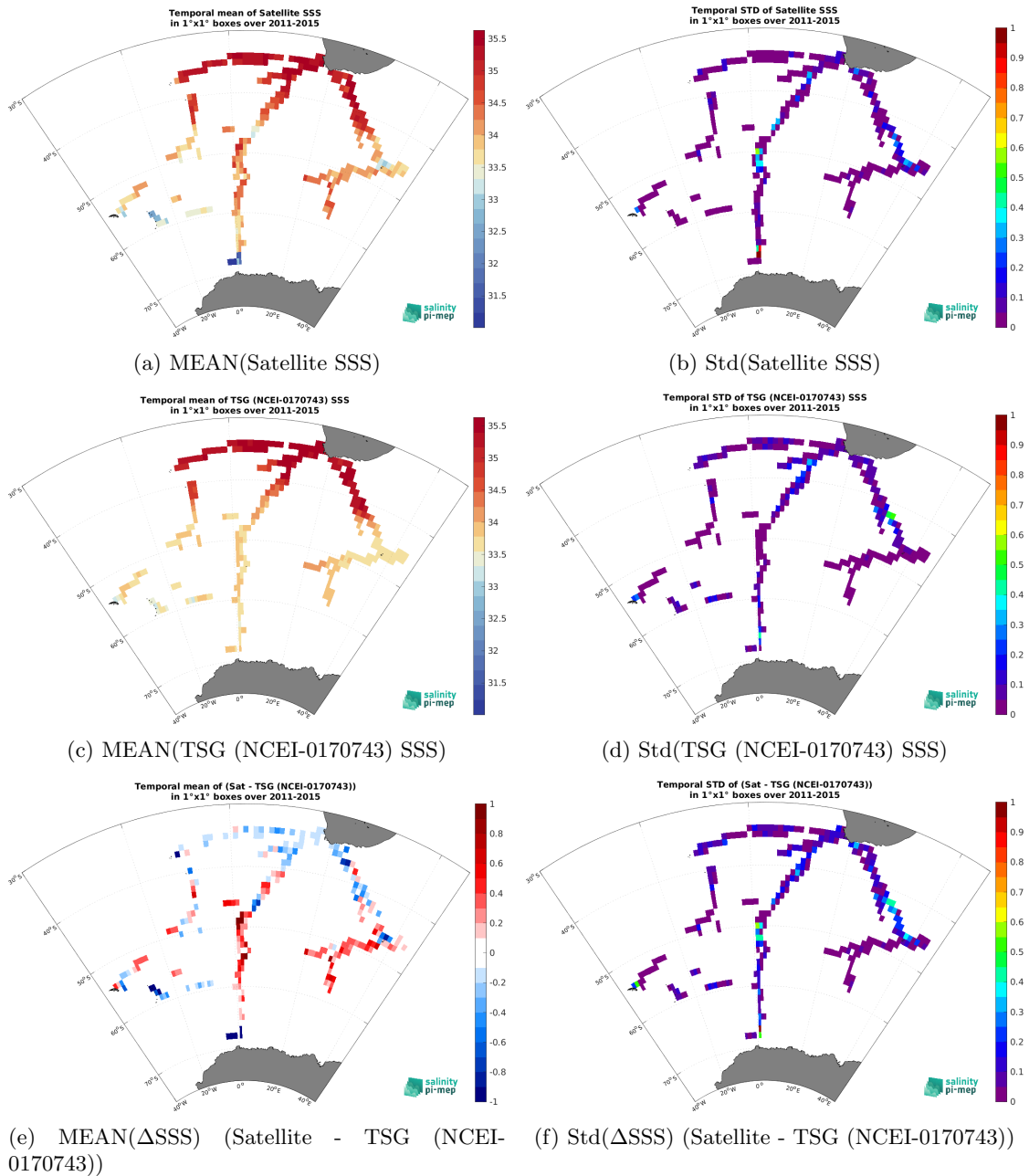
Figure 7: Temporal mean (left) and Std (right) of SSS from Aquarius SSS L3 OR v5 - 7-Day running (NASA-GSFC) (top), TSG (NCEI-0170743) (middle), and of \Delta SSS (Satellite - TSG (NCEI-0170743)). Only match-up pairs are used to generate these maps.
