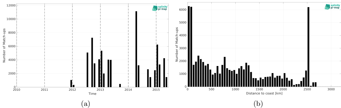
Figure 2: Number of match-ups between TSG (NCEI-0170743) and Aquarius SSS L3 OR v5 - 7-Day running (NASA-GSFC) SSS as a function of time (a) and as function of the distance to coast (b) over the Global Ocean Pi-MEP region and for the full satellite product period.
