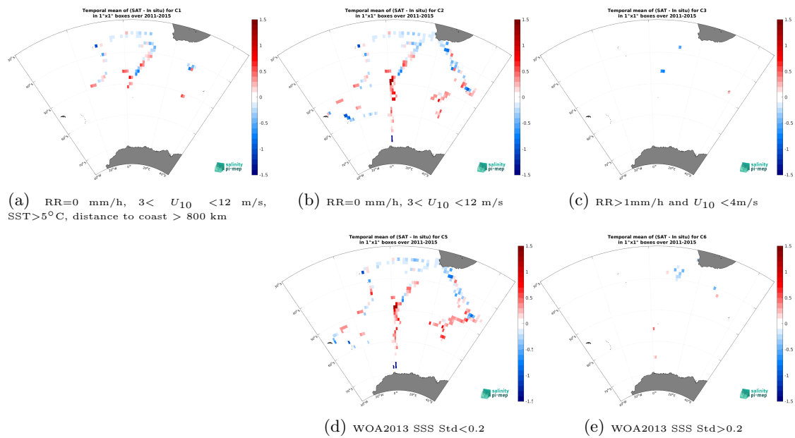
Figure 14: Temporal mean gridded over spatial boxes of size 1^\circ \times 1^\circ of \Delta SSS (Aquarius SSS L3 OR v5 - 7-Day running (NASA-GSFC) - TSG (NCEI-0170743)) for 5 different subdatasets corresponding to:RR=0 mm/h, 3 < U_{10} < 12 m/s, SST >5^\circ\text{C} , distance to coast > 800 km (a), RR=0 mm/h, 3 < U_{10} < 12 m/s (b), RR >1 mm/h and U_{10} < 4 m/s (c), WOA2013 SSS Std <0.2 (d), WOA2013 SSS Std >0.2 (e).
