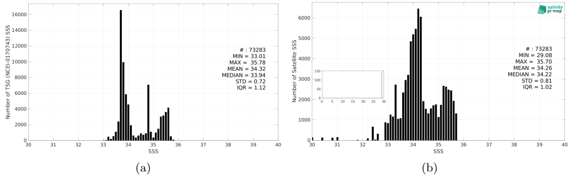
Figure 3: Histograms of SSS from TSG (NCEI-0170743) (a) and Aquarius SSS L3 OR v5 - 7-Day running (NASA-GSFC) (b) considering all match-up pairs per bins of 0.1 over the Global Ocean Pi-MEP region and for the full satellite product period.
