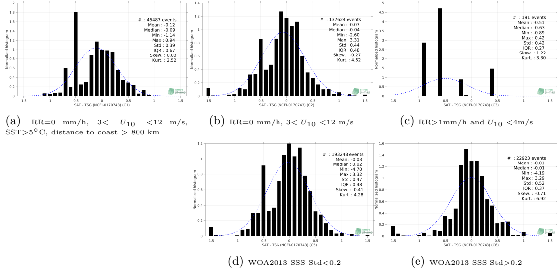
Figure 13: Normalized histogram of \Delta SSS (Aquarius SSS L3 OR v5 - 7-Day running (NASA-GSFC) - TSG (NCEI-0170743)) for 5 different subdatasets corresponding to: RR=0 mm/h, 3 < U_{10} < 12 m/s, SST>5°C, distance to coast > 800 km (a), RR=0 mm/h, 3 < U_{10} < 12 m/s (b), RR>1mm/h and U_{10} < 4 m/s (c), WOA2013 SSS Std<0.2 (d), WOA2013 SSS Std>0.2 (e).
