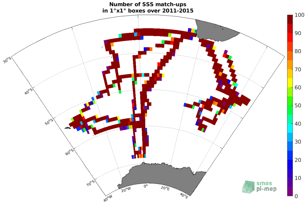
Figure 4: Number of SSS match-ups between TSG (NCEI-0170743) SSS and the Aquarius SSS L3 OR v5 - 7-Day running (NASA-GSFC) SSS product for the Global Ocean Pi-MEP region over 1°x1° boxes and for the full satellite product period.
