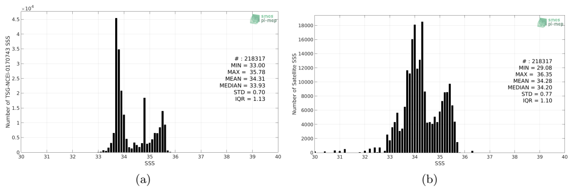
Figure 2: Histograms of SSS from TSG-NCEI-0170743 (a) and Aquarius-L3-OR-V5-7DAY-RUNNING-1DEG (b) considering all match-up pairs per bins of 0.1 over the Global Ocean Pi-MEP region and for the full satellite product period.
