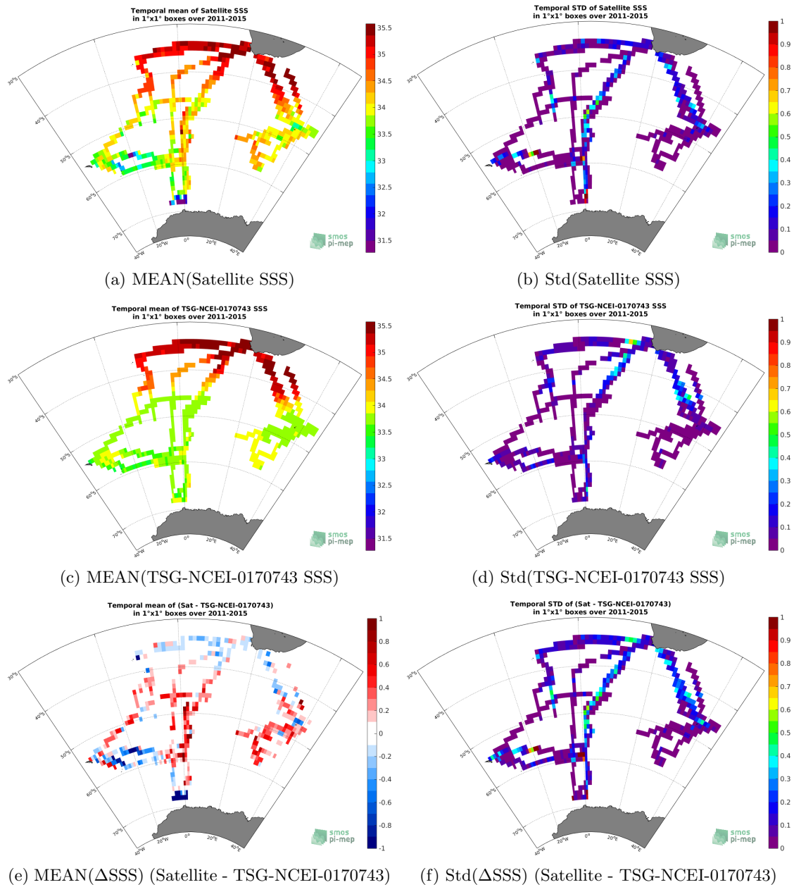
Figure 6: Temporal mean (left) and Std (right) of SSS from Aquarius-L3-OR-V5-7DAY-RUNNING-1DEG (top), TSG-NCEI-0170743 (middle), and of \Delta SSS (Satellite - TSG-NCEI-0170743). Only match-up pairs are used to generate these maps.
