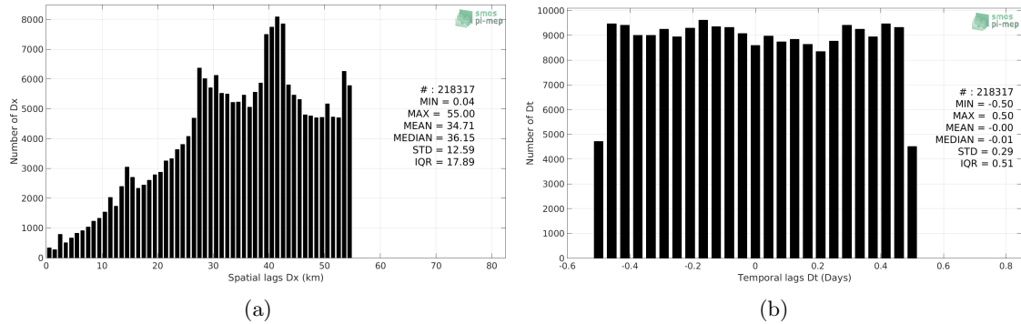
Figure 5: Histograms of the spatial (a) and temporal (b) lags between the time of the TSG-NCEI-0170743 measurements and the date of the corresponding Aquarius-L3-OR-V5-7DAY-RUNNING-1DEG SSS product.
