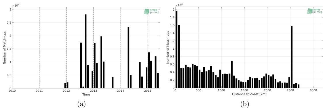
Figure 1: Number of match-ups between TSG-NCEI-0170743 and Aquarius-L3-OR-V5-7DAY-RUNNING-1DEG SSS as a function of time (a) and as function of the distance to coast (b) over the Global Ocean Pi-MEP region and for the full satellite product period.
