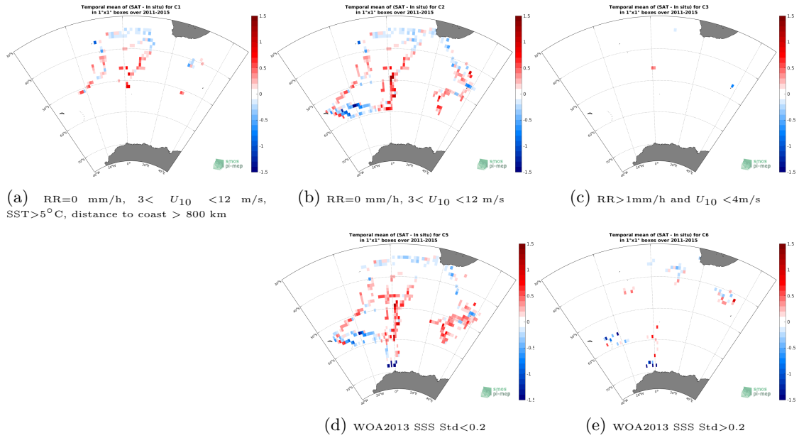
Figure 12: Temporal mean gridded over spatial boxes of size 1^\circ \times 1^\circ of \Delta SSS (Aquarius-L3-OR-V5-7DAY-RUNNING-1DEG - TSG-NCEI-0170743) for 5 different subdatasets corresponding to:RR=0 mm/h, 3 < U_{10} < 12 m/s, SST >5^\circ C, distance to coast > 800 km (a), RR=0 mm/h, 3 < U_{10} < 12 m/s (b), RR >1 mm/h and U_{10} < 4 m/s (c), WOA2013 SSS Std <0.2 (d), WOA2013 SSS Std >0.2 (e).
