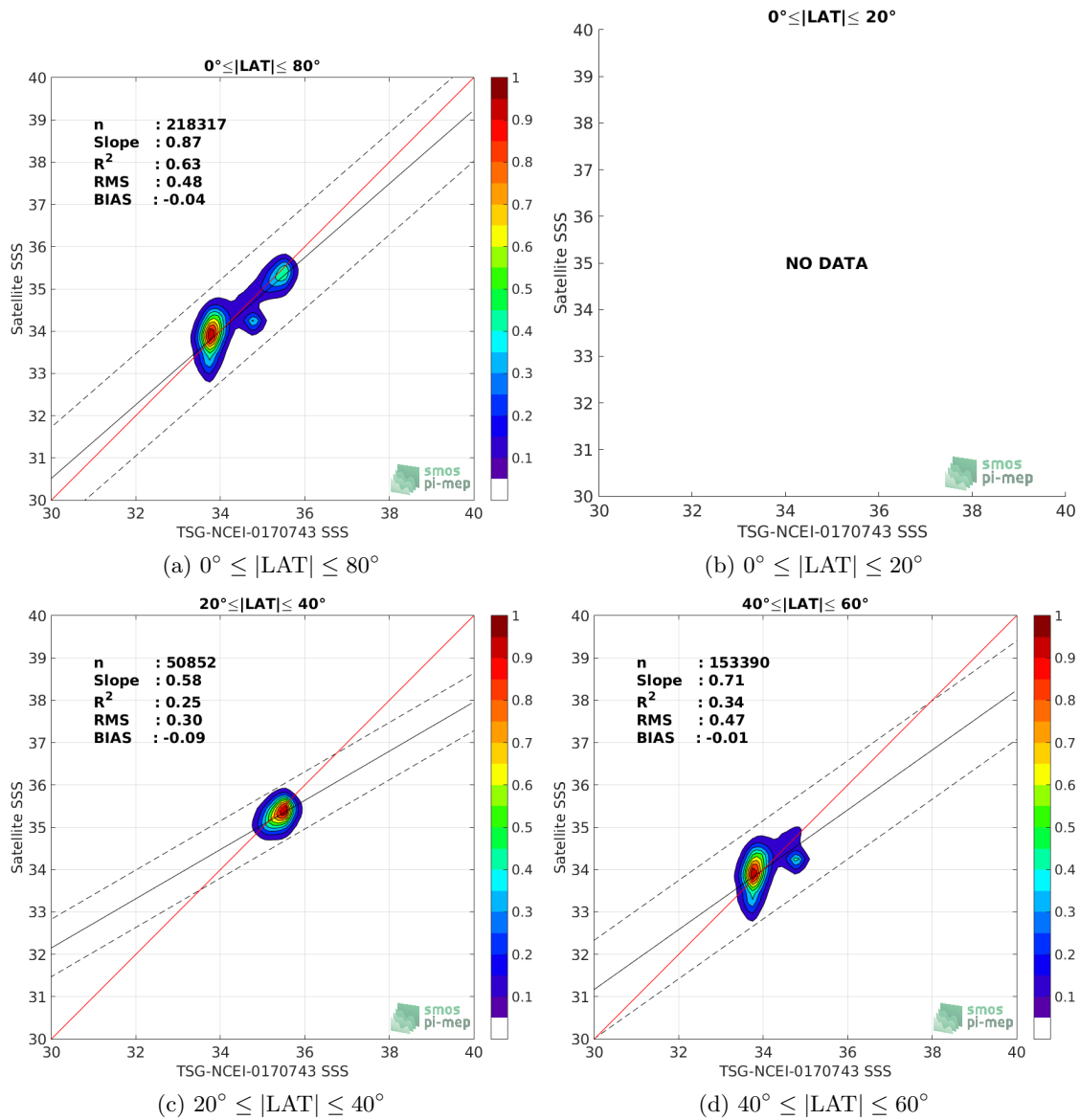
Figure 9: Contour maps of the concentration of Aquarius-L3-OR-V5-7DAY-RUNNING-1DEG SSS (y-axis) versus TSG-NCEI-0170743 SSS (x-axis) at match-up pairs for different latitude bands. For each plot, the red line shows x=y . The black thin and dashed lines indicate a linear fit through the data cloud and the \pm 95\% confidence levels, respectively. The number match-up pairs n , the slope and R^2 coefficient of the linear fit, the root mean square (RMS) and the mean bias between satellite and in situ data are indicated for each latitude band in each plots.
