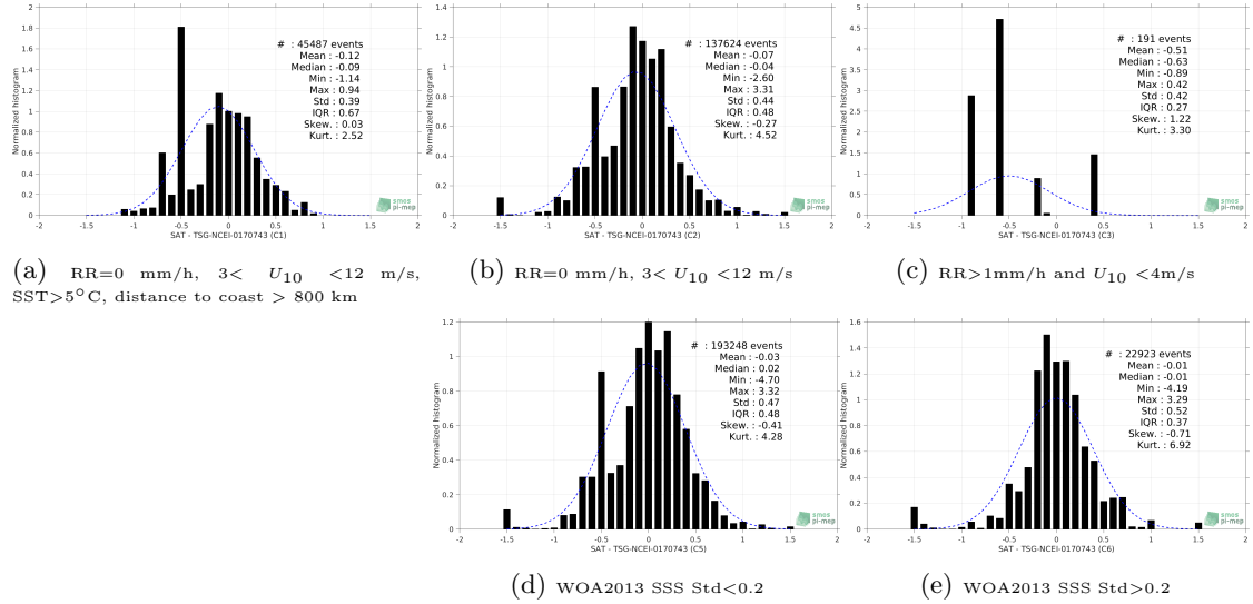
Figure 13: Normalized histogram of \Delta SSS (Aquarius-L3-OR-V5-7DAY-RUNNING-1DEG - TSG-NCEI-0170743) for 5 different subdatasets corresponding to: RR=0 mm/h, 3 < U_{10} < 12 m/s, SST > 5°C, distance to coast > 800 km (a), RR=0 mm/h, 3 < U_{10} < 12 m/s (b), RR > 1mm/h and U_{10} < 4 m/s (c), WOA2013 SSS Std < 0.2 (d), WOA2013 SSS Std > 0.2 (e).
