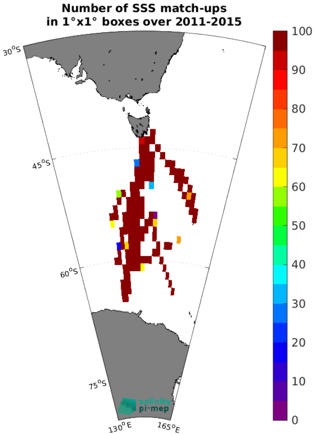
Figure 5: Number of SSS match-ups between TSG (LEGOS-Survostral) SSS and the Aquarius SSS L3 OR v5 - 7-Day running (NASA-GSFC) SSS product for the Global Ocean Pi-MEP region over 1°x1° boxes and for the full satellite product period.
