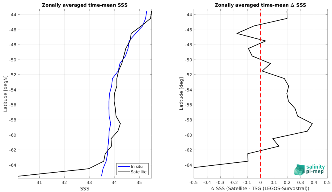
Figure 9: Left panel: Zonal mean SSS from Aquarius SSS L3 OR v5 - 7-Day running (NASA-GSFC) satellite product (black) and from TSG (LEGOS-Survostral) (blue). Right panel: Zonal mean of \Delta SSS (Satellite - TSG (LEGOS-Survostral)) for all the collected Pi-MEP match-up pairs estimated over the full satellite product period.
