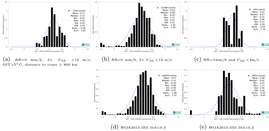
Figure 15: Normalized histogram of \Delta SSS (Aquarius SSS L3 OR v5 - 7-Day running (NASA-GSFC) - TSG (LEGOS-Survostral)) for 5 different subdatasets corresponding to: RR=0 mm/h, 3 < U_{10} < 12 m/s, SST > 5°C, distance to coast > 800 km (a), RR=0 mm/h, 3 < U_{10} < 12 m/s (b), RR > 1mm/h and U_{10} < 4 m/s (c), WOA2013 SSS Std < 0.2 (d), WOA2013 SSS Std > 0.2 (e).
