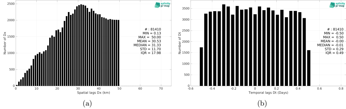
Figure 6: Histograms of the spatial (a) and temporal (b) lags between the location/time of the TSG (LEGOS-Survostral) measurement and the date of the corresponding Aquarius SSS L3 OR v5 - 7-Day running (NASA-GSFC) SSS pixel.
