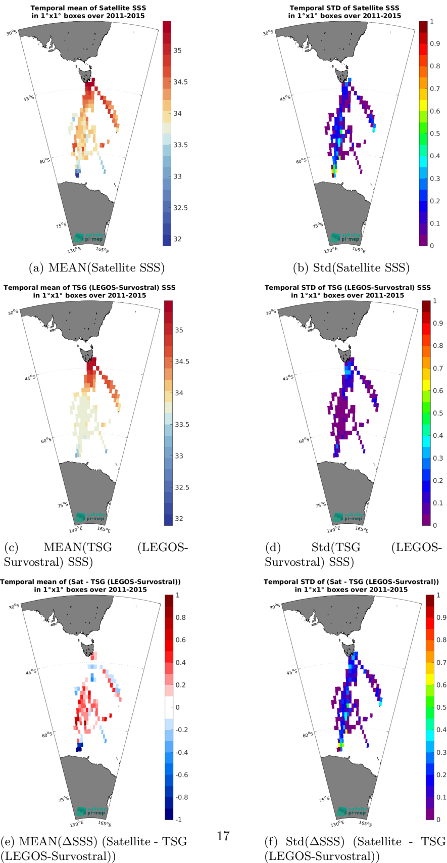
Figure 7: Temporal mean (left) and Std (right) of SSS from Aquarius SSS L3 OR v5 - 7-Day running (NASA-GSFC) (top), TSG (LEGOS-Survostral) (middle), and of \Delta SSS (Satellite - TSG (LEGOS-Survostral)). Only match-up pairs are used to generate these maps.
