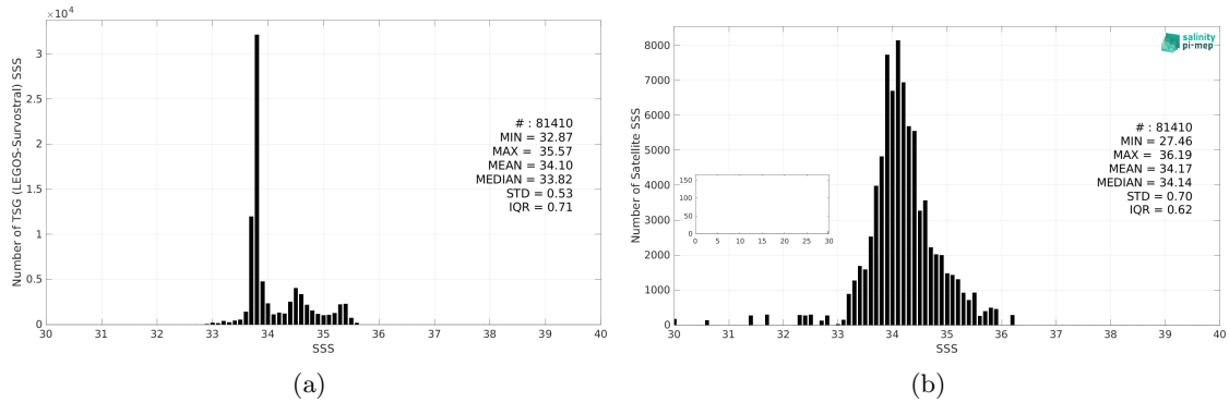
Figure 3: Histograms of SSS from TSG (LEGOS-Survostral) (a) and Aquarius SSS L3 OR v5 - 7-Day running (NASA-GSFC) (b) considering all match-up pairs per bins of 0.1 over the Global Ocean Pi-MEP region and for the full satellite product period.
