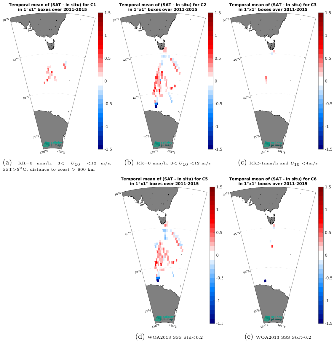
Figure 14: Temporal mean gridded over spatial boxes of size 1^\circ \times 1^\circ of \Delta\text{SSS} (Aquarius SSS L3 OR v5 - 7-Day running (NASA-GSFC) - TSG (LEGOS-Survostral)) for 5 different subdatasets corresponding to: RR=0 mm/h, 3 < U_{10} < 12 m/s, SST > 5^\circ\text{C} , distance to coast > 800 km (a), RR=0 mm/h, 3 < U_{10} < 12 m/s (b), RR > 1 mm/h and U_{10} < 4 m/s (c), WOA2013 SSS Std < 0.2 (d), WOA2013 SSS Std > 0.2 (e).
