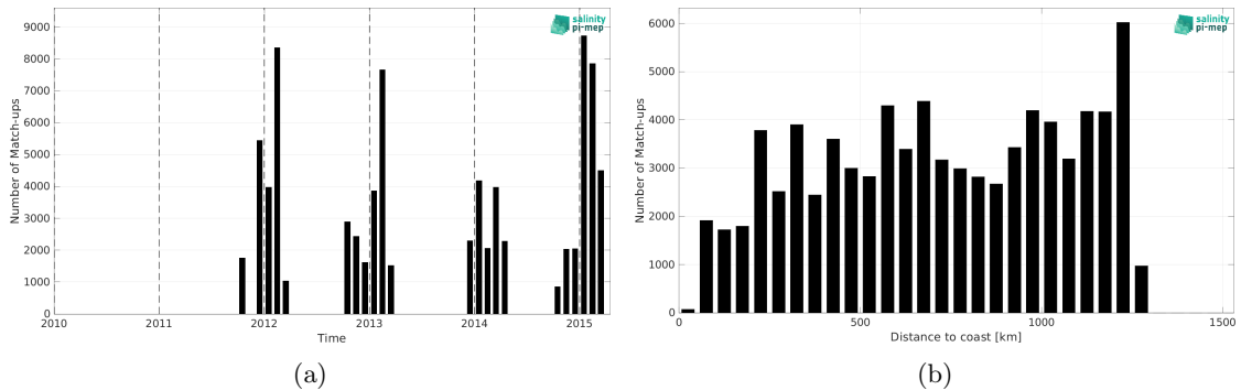
Figure 2: Number of match-ups between TSG (LEGOS-Survostral) and Aquarius SSS L3 OR v5 - 7-Day running (NASA-GSFC) SSS as a function of time (a) and as function of the distance to coast (b) over the Global Ocean Pi-MEP region and for the full satellite product period.
