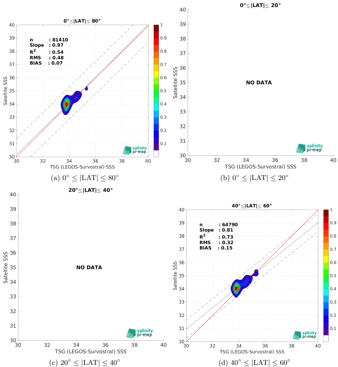
Figure 10: Contour maps of the concentration of Aquarius SSS L3 OR v5 - 7-Day running (NASA-GSFC) SSS (y-axis) versus TSG (LEGOS-Survostral) SSS (x-axis) at match-up pairs for different latitude bands. For each plot, the red line shows x=y . The black thin and dashed lines indicate a linear fit through the data cloud and the \pm 95\% confidence levels, respectively. The number match-up pairs n , the slope and R^2 coefficient of the linear fit, the root mean square (RMS) and the mean bias between satellite and in situ data are indicated for each latitude band in each plots.
