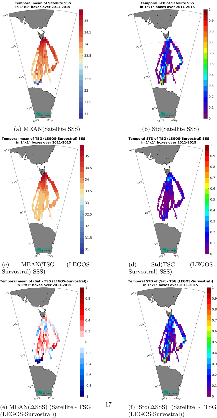
Figure 6: Temporal mean (left) and Std (right) of SSS from Aquarius SSS L3 OR v5 - 7-Day running (NASA-GSFC) (top), TSG (LEGOS-Survostral) (middle), and of \Delta SSS (Satellite - TSG (LEGOS-Survostral)). Only match-up pairs are used to generate these maps.
