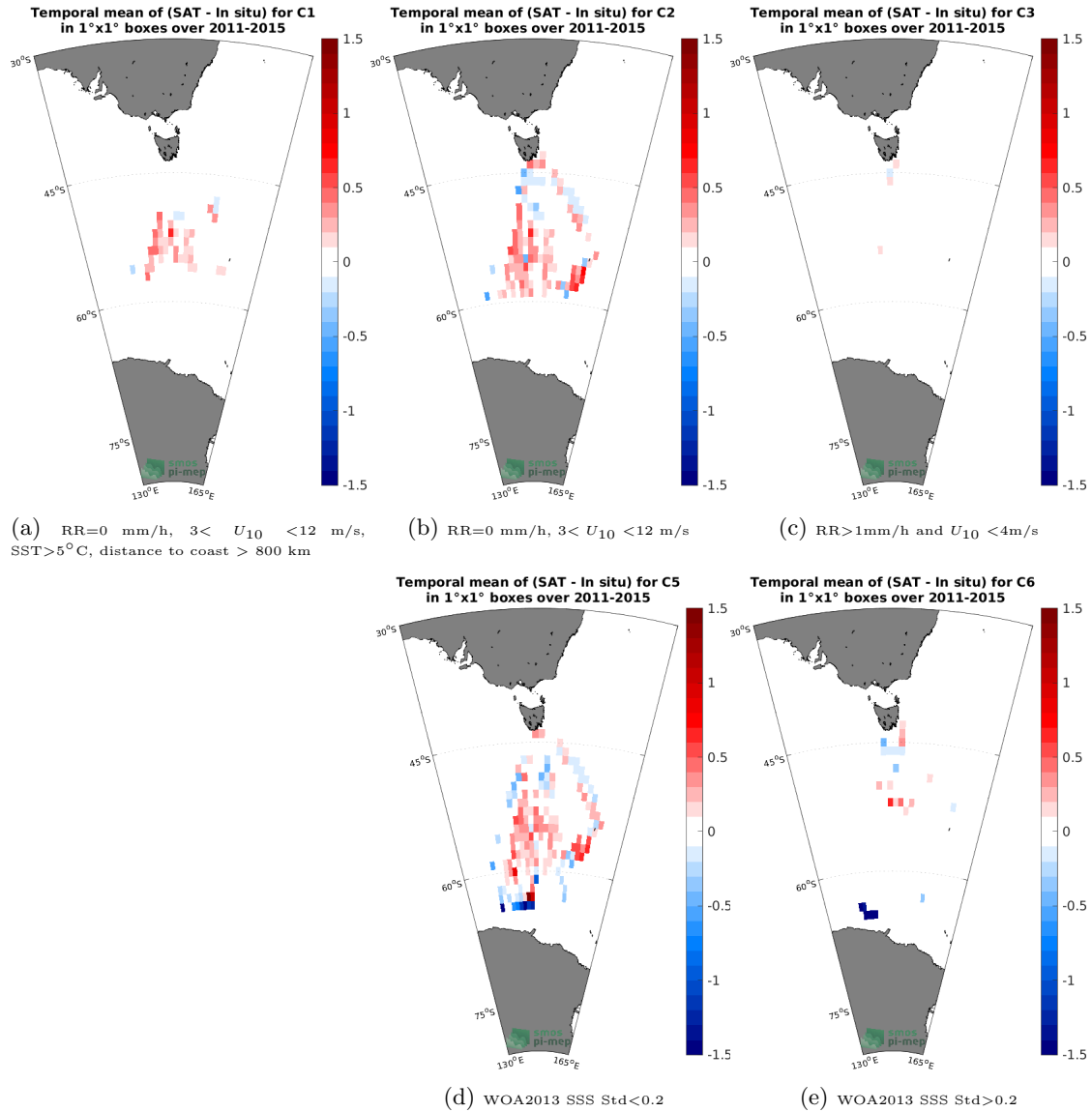
Figure 12: Temporal mean gridded over spatial boxes of size 1^\circ \times 1^\circ of \Delta SSS (Aquarius SSS L3 OR v5 - 7-Day running (NASA-GSFC) - TSG (LEGOS-Survostral)) for 5 different subdatasets corresponding to: RR=0 mm/h, 3 < U_{10} < 12 m/s, SST > 5°C, distance to coast > 800 km (a), RR=0 mm/h, 3 < U_{10} < 12 m/s (b), RR > 1mm/h and U_{10} < 4 m/s (c), WOA2013 SSS Std < 0.2 (d), WOA2013 SSS Std > 0.2 (e).
