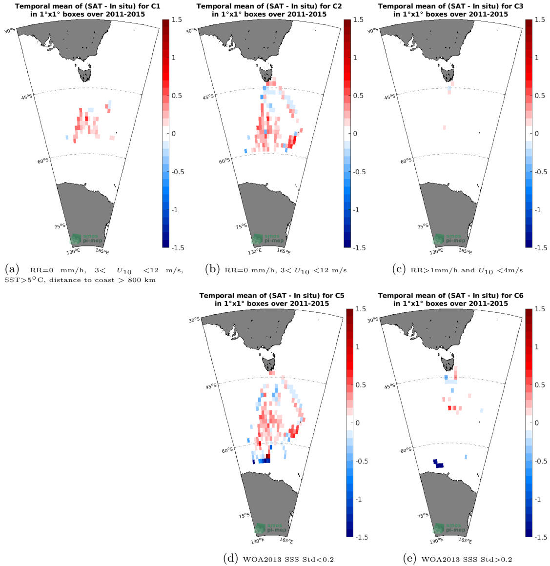
Figure 12: Temporal mean gridded over spatial boxes of size 1°x1° of \Delta SSS (Aquarius SSS L3 OR v5 - 7-Day running (NASA-GSFC) - TSG (LEGOS-Survostral)) for 5 different subdatasets corresponding to:RR=0 mm/h, 3 < U_{10} < 12 m/s, SST>5°C, distance to coast > 800 km (a), RR=0 mm/h, 3 < U_{10} < 12 m/s (b), RR>1mm/h and U_{10} < 4 m/s (c), WOA2013 SSS Std<0.2 (d), WOA2013 SSS Std>0.2 (e).
