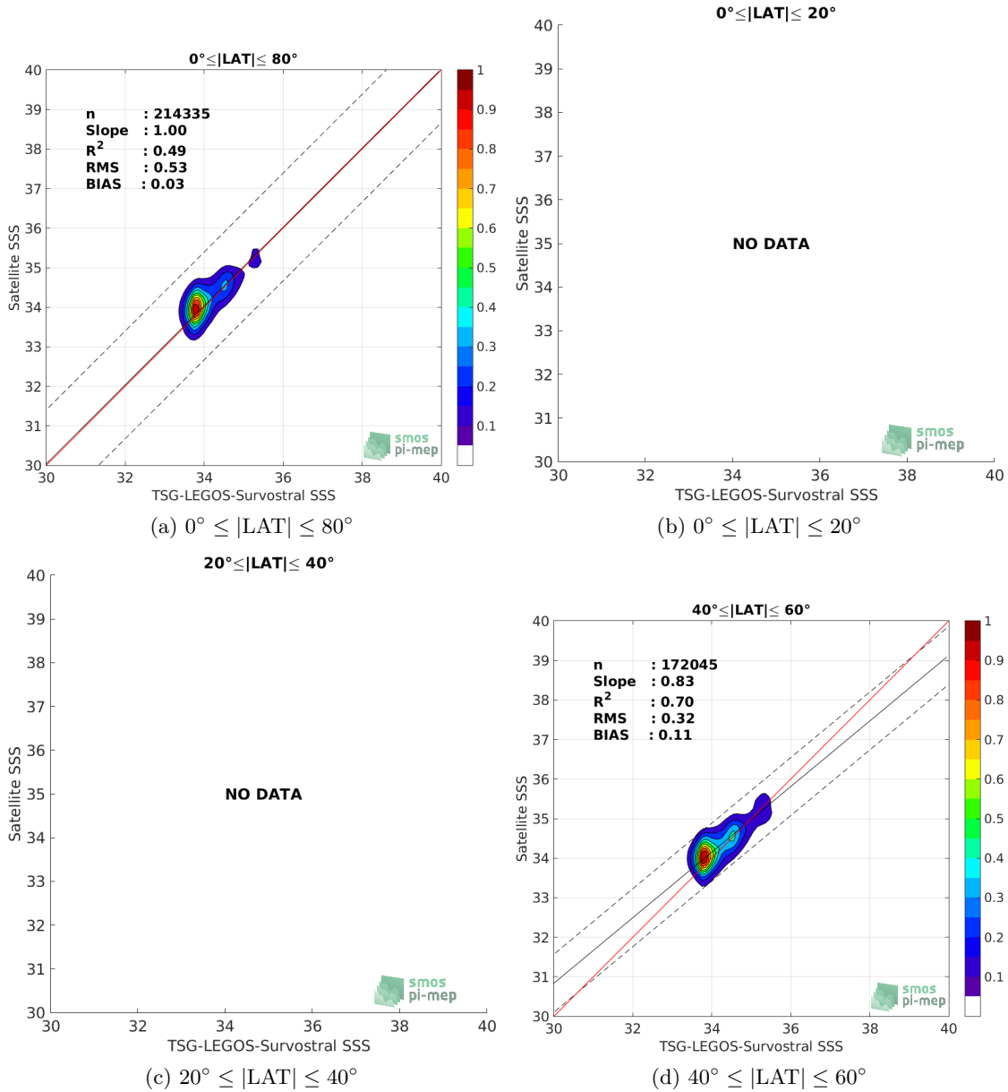
Figure 9: Contour maps of the concentration of Aquarius-L3-OR-V5-7DAY-RUNNING-1DEG SSS (y-axis) versus TSG-LEGOS-Survostral SSS (x-axis) at match-up pairs for different latitude bands. For each plot, the red line shows x=y . The black thin and dashed lines indicate a linear fit through the data cloud and the \pm 95\% confidence levels, respectively. The number match-up pairs n , the slope and R^2 coefficient of the linear fit, the root mean square (RMS) and the mean bias between satellite and in situ data are indicated for each latitude band in each plots.
