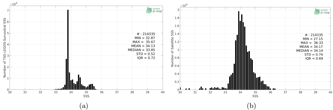
Figure 2: Histograms of SSS from TSG-LEGOS-Survostral (a) and Aquarius-L3-OR-V5-7DAY-RUNNING-1DEG (b) considering all match-up pairs per bins of 0.1 over the Global Ocean Pi-MEP region and for the full satellite product period.
