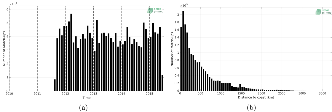
Figure 1: Number of match-ups between TSG (LEGOS-DM) and Aquarius SSS L3 OR v5 - 7-Day running (NASA-GSFC) SSS as a function of time (a) and as function of the distance to coast (b) over the Global Ocean Pi-MEP region and for the full satellite product period.
