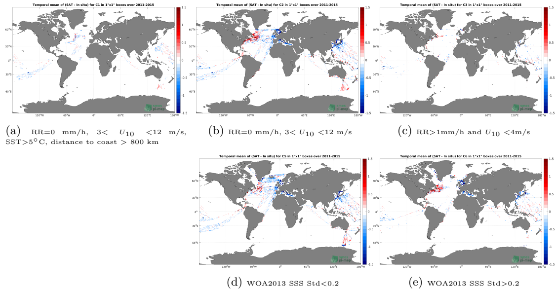
Figure 12: Temporal mean gridded over spatial boxes of size 1^\circ \times 1^\circ of \Delta\text{SSS} (Aquarius SSS L3 OR v5 - 7-Day running (NASA-GSFC) - TSG (LEGOS-DM)) for 5 different subdatasets corresponding to:RR=0 mm/h, 3 < U_{10} < 12 m/s, SST >5^\circ\text{C} , distance to coast > 800 km (a), RR=0 mm/h, 3 < U_{10} < 12 m/s (b), RR >1 mm/h and U_{10} < 4 m/s (c), WOA2013 SSS Std <0.2 (d), WOA2013 SSS Std >0.2 (e).
