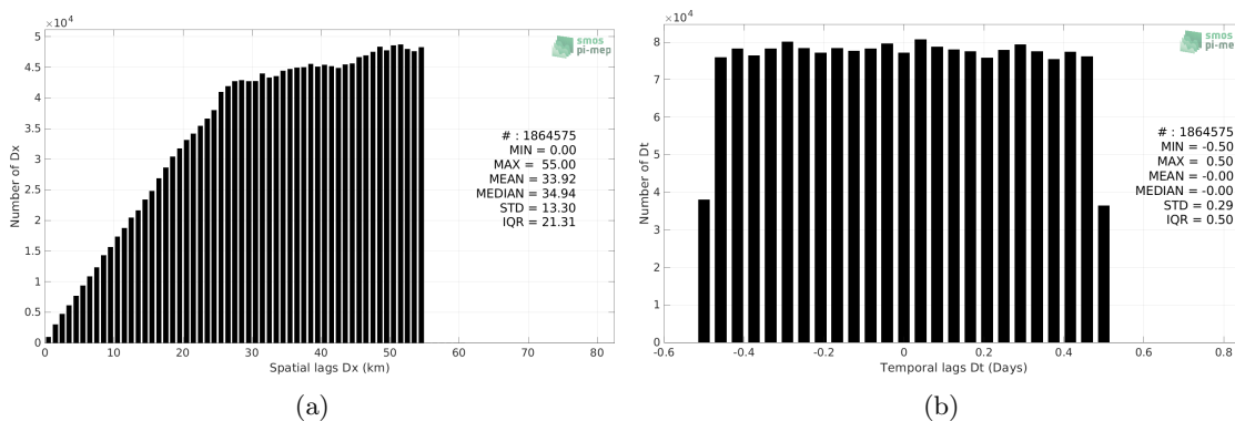
Figure 5: Histograms of the spatial (a) and temporal (b) lags between the location/time of the TSG (LEGOS-DM) measurement and the date of the corresponding Aquarius SSS L3 OR v5 - 7-Day running (NASA-GSFC) SSS pixel.
