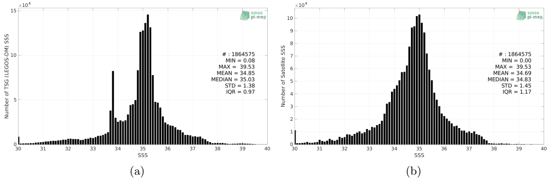
Figure 2: Histograms of SSS from TSG (LEGOS-DM) (a) and Aquarius SSS L3 OR v5 - 7-Day running (NASA-GSFC) (b) considering all match-up pairs per bins of 0.1 over the Global Ocean Pi-MEP region and for the full satellite product period.
