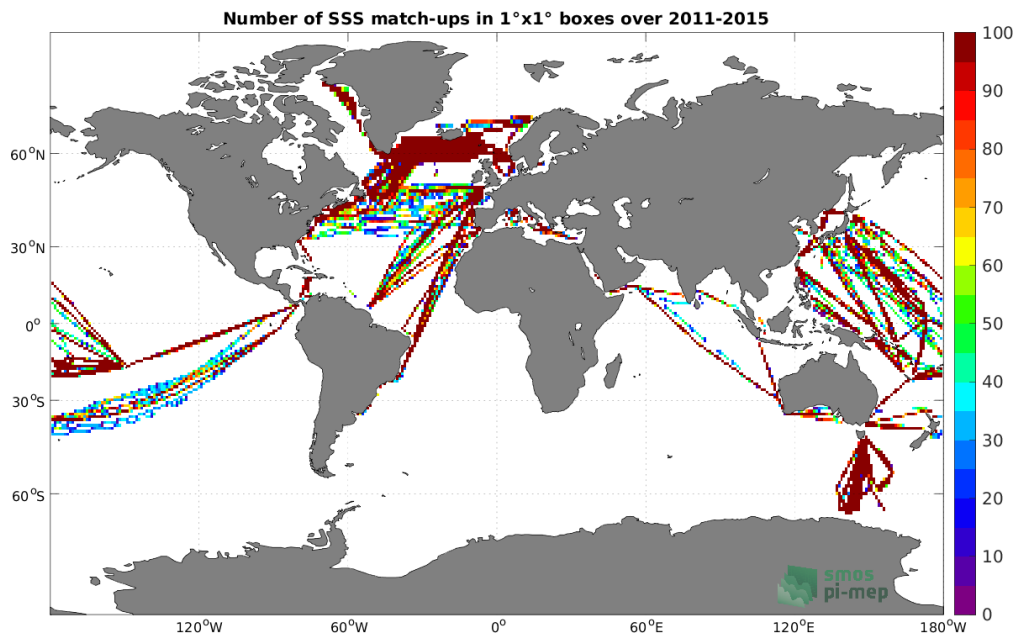
Figure 4: Number of SSS match-ups between TSG (LEGOS-DM) SSS and the Aquarius SSS L3 OR v5 - 7-Day running (NASA-GSFC) SSS product for the Global Ocean Pi-MEP region over 1^\circ \times 1^\circ boxes and for the full satellite product period.
