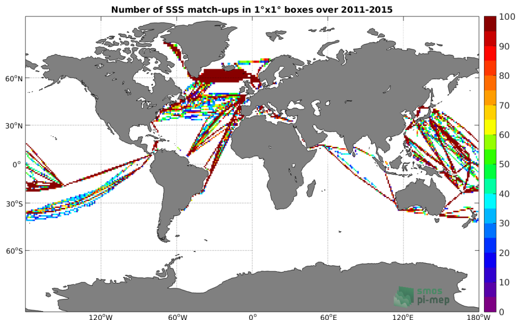
Figure 4: Number of SSS match-ups between TSG (LEGOS-DM) SSS and the Aquarius SSS L3 OR v5 - 7-Day running (NASA-GSFC) SSS product for the Global Ocean Pi-MEP region over 1^\circ \times 1^\circ boxes and for the full satellite product period.
