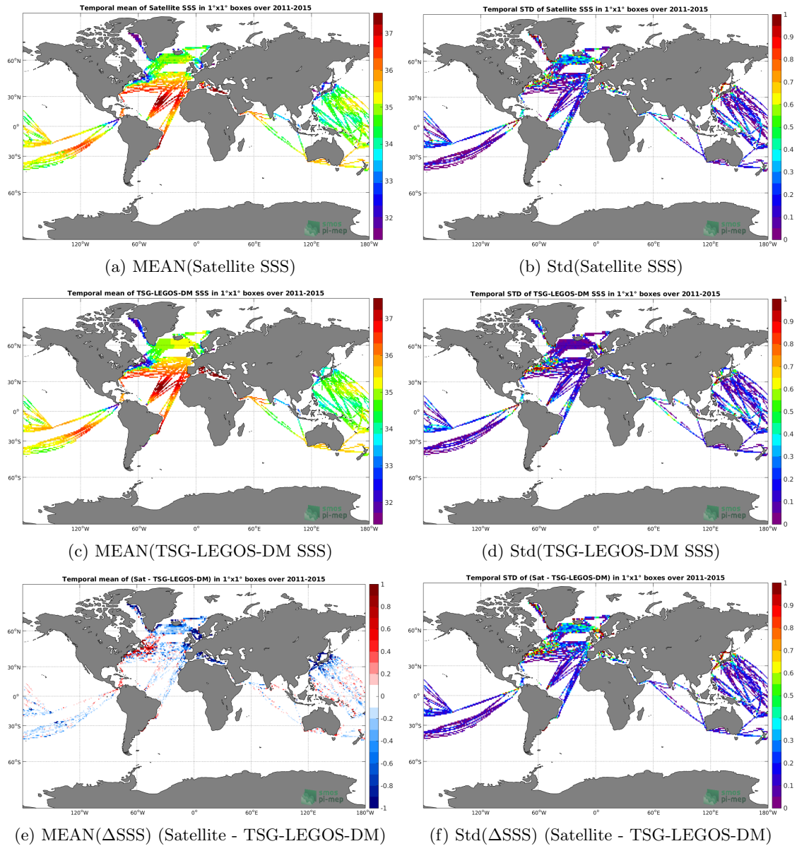
Figure 6: Temporal mean (left) and Std (right) of SSS from Aquarius-L3-OR-V5-7DAY-RUNNING-1DEG (top), TSG-LEGOS-DM (middle), and of \Delta SSS (Satellite - TSG-LEGOS-DM). Only match-up pairs are used to generate these maps.
