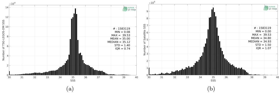
Figure 2: Histograms of SSS from TSG-LEGOS-DM (a) and Aquarius-L3-OR-V5-7DAY-RUNNING-1DEG (b) considering all match-up pairs per bins of 0.1 over the Global Ocean Pi-MEP region and for the full satellite product period.
