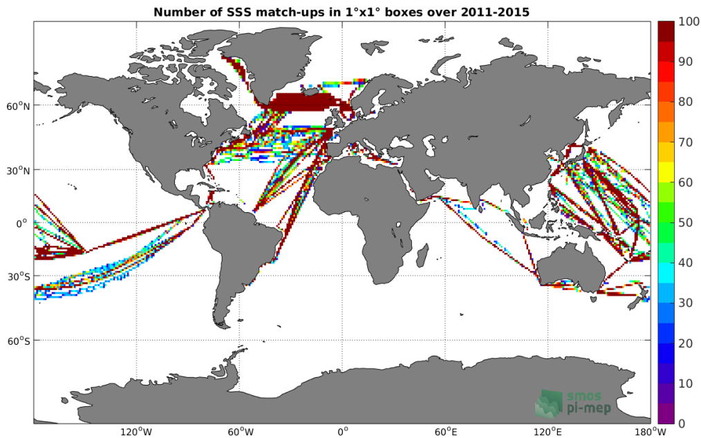
Figure 4: Number of SSS match-ups between TSG-LEGOS-DM SSS and the Aquarius-L3-OR-V5-7DAY-RUNNING-1DEG SSS product for the Global Ocean Pi-MEP region over 1^\circ \times 1^\circ boxes and for the full satellite product period.
