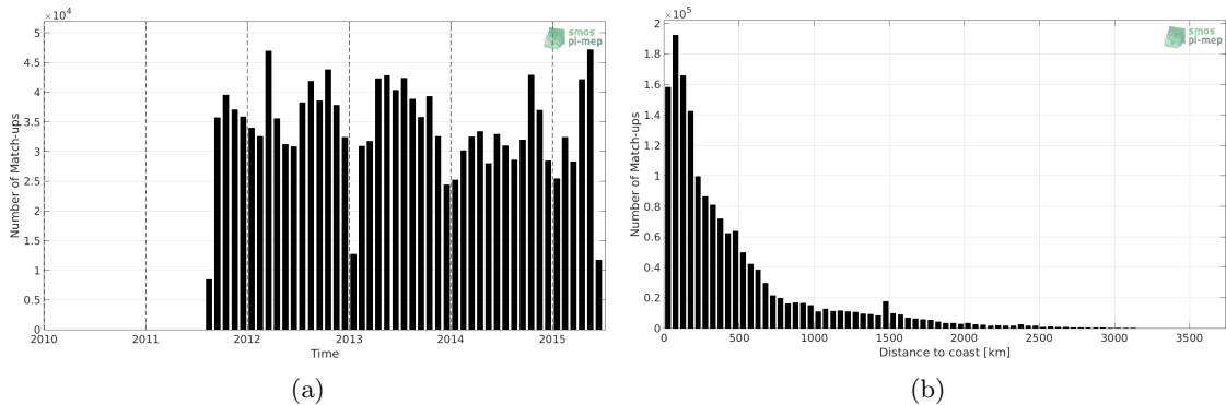
Figure 1: Number of match-ups between TSG-LEGOS-DM and Aquarius-L3-OR-V5-7DAY-RUNNING-1DEG SSS as a function of time (a) and as function of the distance to coast (b) over the Global Ocean Pi-MEP region and for the full satellite product period.
