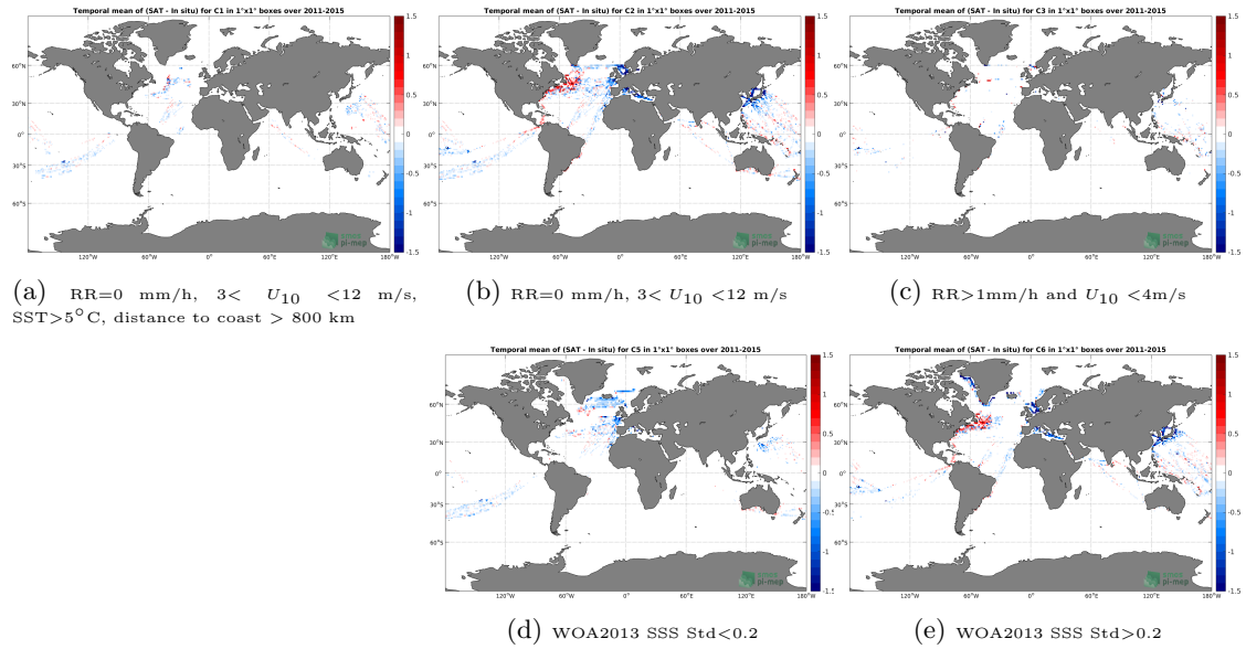
Figure 12: Temporal mean gridded over spatial boxes of size 1^\circ \times 1^\circ of \Delta SSS (Aquarius-L3-OR-V5-7DAY-RUNNING-1DEG - TSG-LEGOS-DM) for 5 different subdatasets corresponding to: RR=0 mm/h, 3 < U_{10} < 12 m/s, SST > 5^\circ C, distance to coast > 800 km (a), RR=0 mm/h, 3 < U_{10} < 12 m/s (b), RR > 1 mm/h and U_{10} < 4 m/s (c), WOA2013 SSS Std < 0.2 (d), WOA2013 SSS Std > 0.2 (e).
