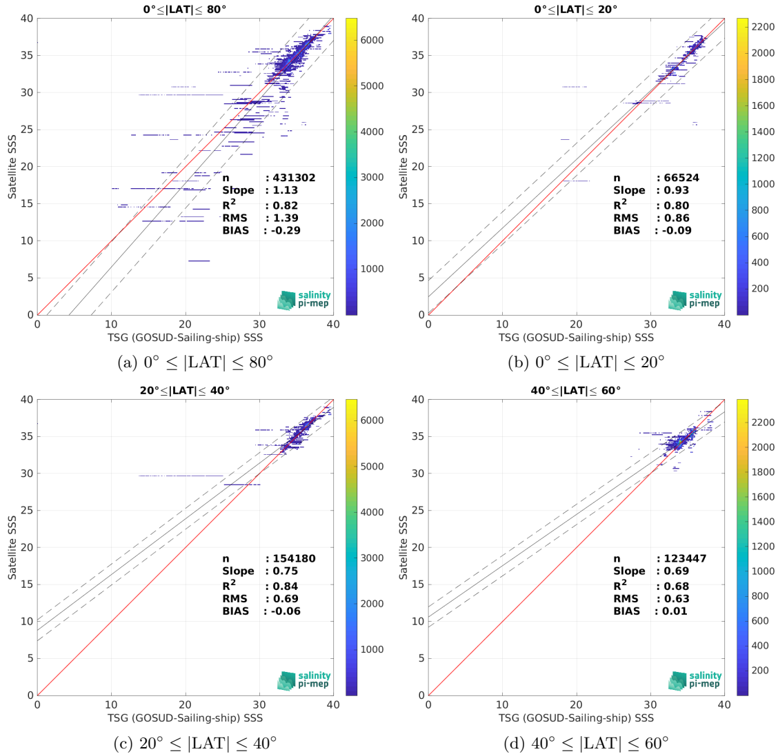
Figure 9: Contour maps of the concentration of Aquarius SSS L3 OR v5 - 7-Day running (NASA-GSFC) SSS (y-axis) versus TSG (GOSUD-Sailing-ship) SSS (x-axis) at match-up pairs for different latitude bands. For each plot, the red line shows x=y . The black thin and dashed lines indicate a linear fit through the data cloud and the \pm 95\% confidence levels, respectively. The number match-up pairs n , the slope and R^2 coefficient of the linear fit, the root mean square (RMS) and the mean bias between satellite and in situ data are indicated for each latitude band in each plots.
