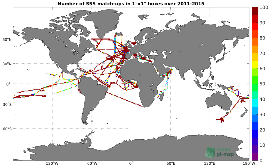
Figure 4: Number of SSS match-ups between TSG (GOSUD-Research-vessel) SSS and the Aquarius SSS L3 OR v5 - 7-Day running (NASA-GSFC) SSS product for the Global Ocean Pi-MEP region over 1^\circ \times 1^\circ boxes and for the full satellite product period.
