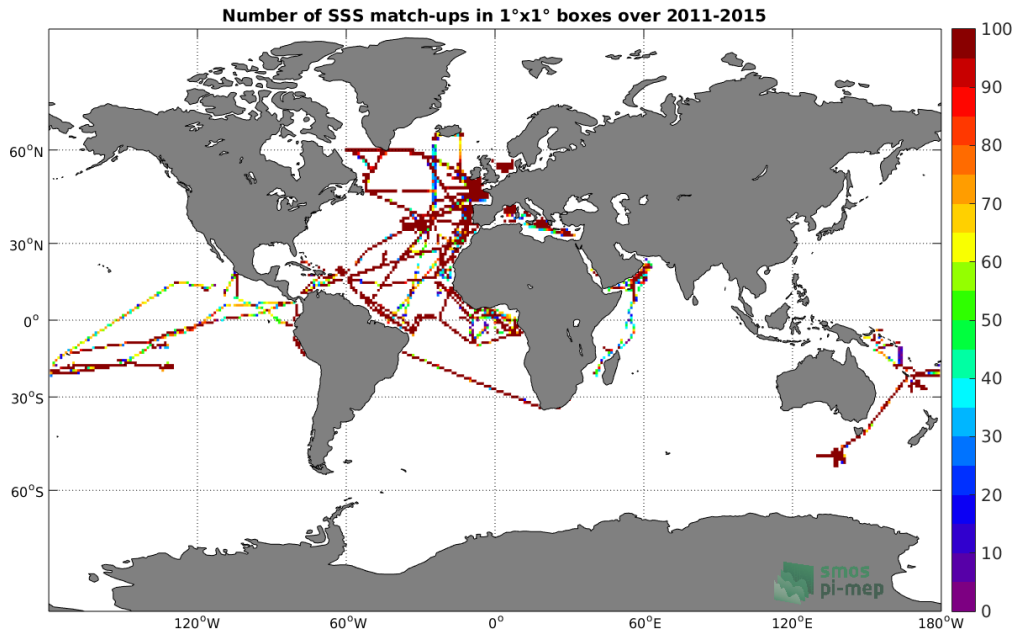
Figure 4: Number of SSS match-ups between TSG-GOSUD-Research-vessel SSS and the Aquarius-L3-OR-V5-7DAY-RUNNING-1DEG SSS product for the Global Ocean Pi-MEP region over 1°x1° boxes and for the full satellite product period.
