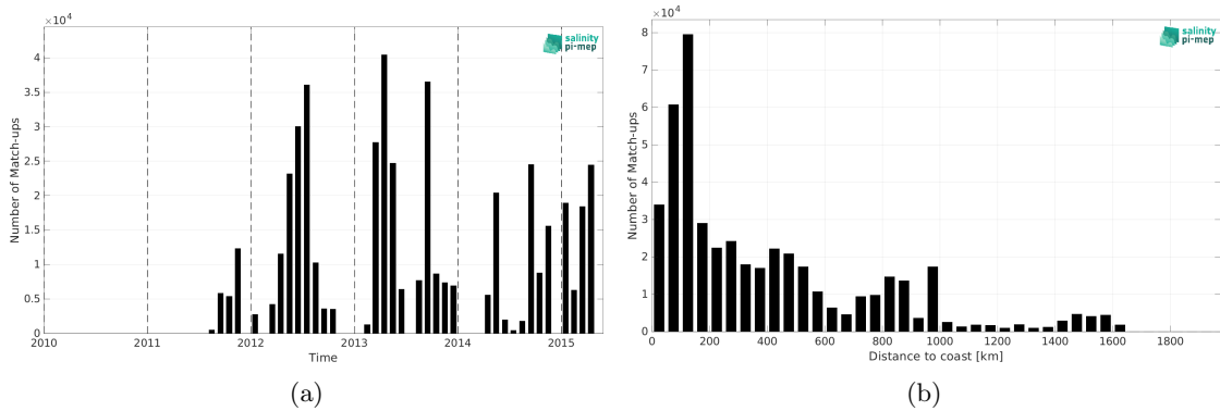
Figure 1: Number of match-ups between TSG (CSIC-UTM) and Aquarius SSS L3 OR v5 - 7-Day running (NASA-GSFC) SSS as a function of time (a) and as function of the distance to coast (b) over the Global Ocean Pi-MEP region and for the full satellite product period.
