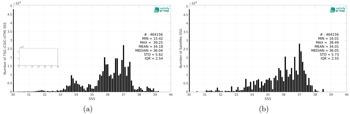
Figure 2: Histograms of SSS from TSG (CSIC-UTM) (a) and Aquarius SSS L3 OR v5 - 7-Day running (NASA-GSFC) (b) considering all match-up pairs per bins of 0.1 over the Global Ocean Pi-MEP region and for the full satellite product period.
