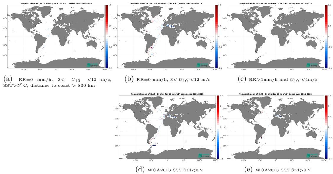
Figure 12: Temporal mean gridded over spatial boxes of size 1^\circ \times 1^\circ of \Delta SSS (Aquarius SSS L3 OR v5 - 7-Day running (NASA-GSFC) - TSG (CSIC-UTM)) for 5 different subdatasets corresponding to: RR=0 mm/h, 3 < U_{10} < 12 m/s, SST > 5^\circ\text{C} , distance to coast > 800 km (a), RR=0 mm/h, 3 < U_{10} < 12 m/s (b), RR > 1 mm/h and U_{10} < 4 m/s (c), WOA2013 SSS Std < 0.2 (d), WOA2013 SSS Std > 0.2 (e).
