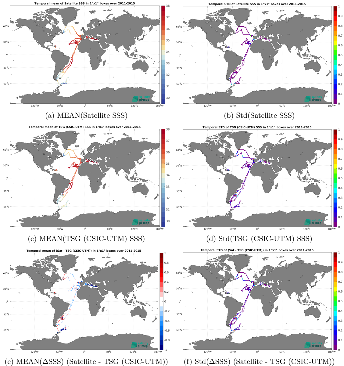
Figure 6: Temporal mean (left) and Std (right) of SSS from Aquarius SSS L3 OR v5 - 7-Day running (NASA-GSFC) (top), TSG (CSIC-UTM) (middle), and of \Delta SSS (Satellite - TSG (CSIC-UTM)). Only match-up pairs are used to generate these maps.
