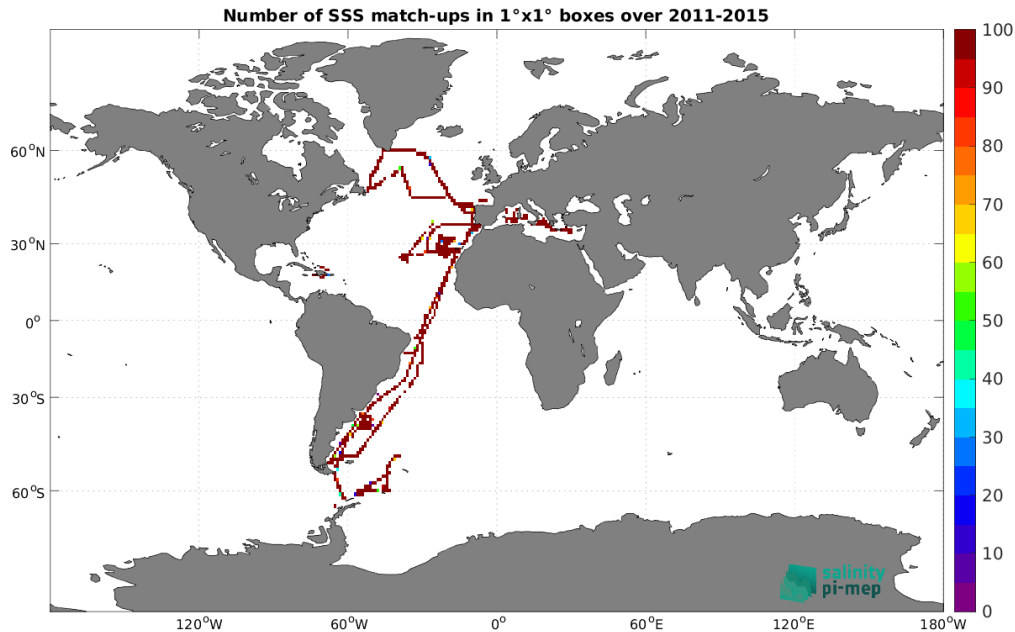
Figure 4: Number of SSS match-ups between TSG (CSIC-UTM) SSS and the Aquarius SSS L3 OR v5 - 7-Day running (NASA-GSFC) SSS product for the Global Ocean Pi-MEP region over 1^\circ \times 1^\circ boxes and for the full satellite product period.
