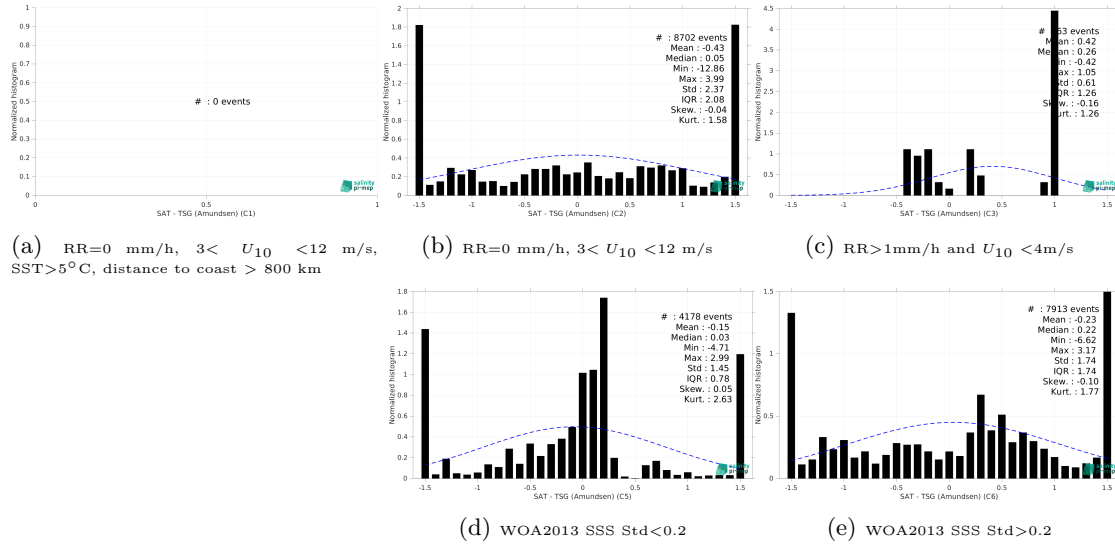
Figure 15: Normalized histogram of \Delta SSS (Aquarius SSS L3 OR v5 - 7-Day running (NASA-GSFC) - TSG (Amundsen)) for 5 different subdatasets corresponding to: RR=0 mm/h, 3 < U_{10} < 12 m/s, SST > 5°C, distance to coast > 800 km (a), RR=0 mm/h, 3 < U_{10} < 12 m/s (b), RR > 1mm/h and U_{10} < 4 m/s (c), WOA2013 SSS Std < 0.2 (d), WOA2013 SSS Std > 0.2 (e).
