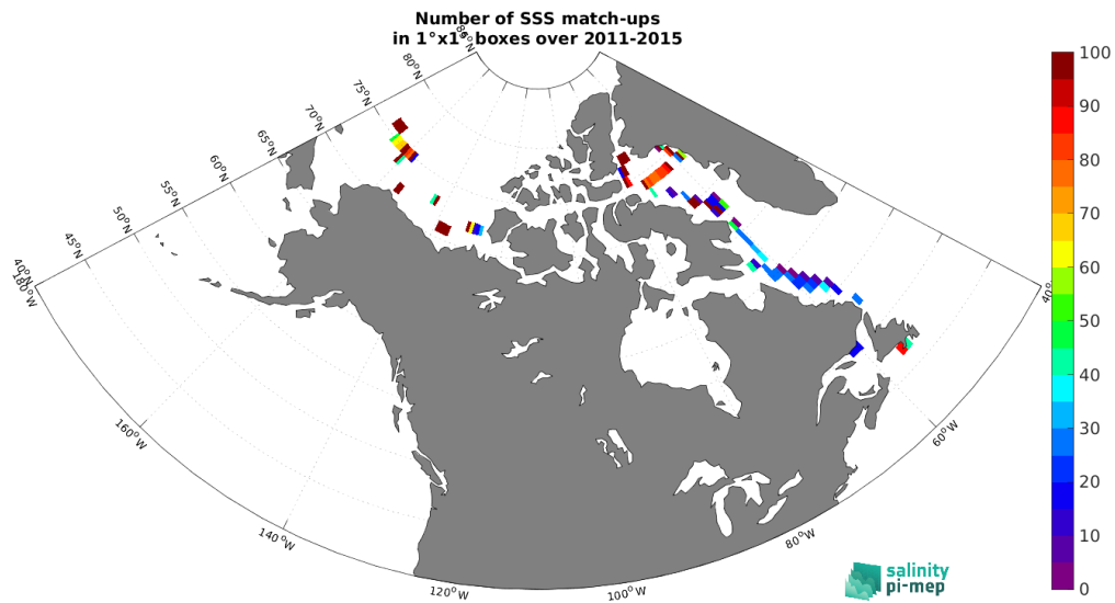
Figure 5: Number of SSS match-ups between TSG (Amundsen) SSS and the Aquarius SSS L3 OR v5 - 7-Day running (NASA-GSFC) SSS product for the Global Ocean Pi-MEP region over 1°×1° boxes and for the full satellite product period.
