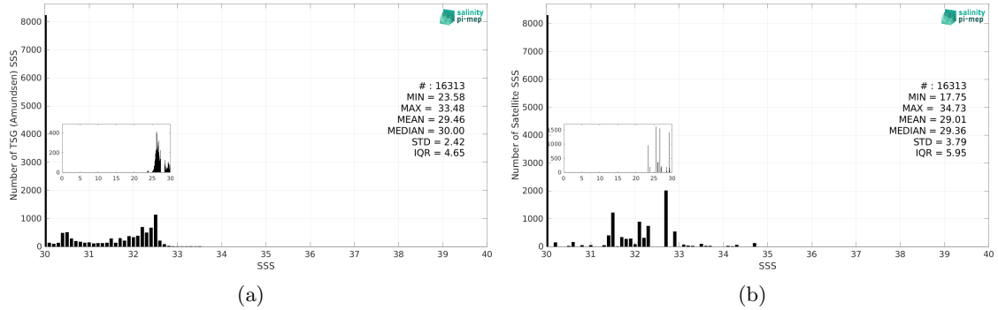
Figure 3: Histograms of SSS from TSG (Amundsen) (a) and Aquarius SSS L3 OR v5 - 7-Day running (NASA-GSFC) (b) considering all match-up pairs per bins of 0.1 over the Global Ocean Pi-MEP region and for the full satellite product period.
