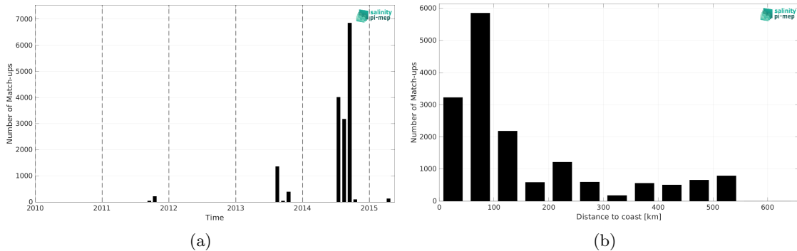
Figure 2: Number of match-ups between TSG (Amundsen) and Aquarius SSS L3 OR v5 - 7-Day running (NASA-GSFC) SSS as a function of time (a) and as function of the distance to coast (b) over the Global Ocean Pi-MEP region and for the full satellite product period.
