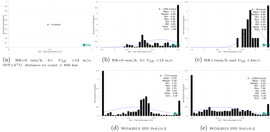
Figure 13: Normalized histogram of \Delta SSS (Aquarius SSS L3 OR v5 - 7-Day running (NASA-GSFC) - TSG (Amundsen)) for 5 different subdatasets corresponding to: RR=0 mm/h, 3 < U_{10} < 12 m/s, SST > 5°C, distance to coast > 800 km (a), RR=0 mm/h, 3 < U_{10} < 12 m/s (b), RR > 1mm/h and U_{10} < 4 m/s (c), WOA2013 SSS Std < 0.2 (d), WOA2013 SSS Std > 0.2 (e).
