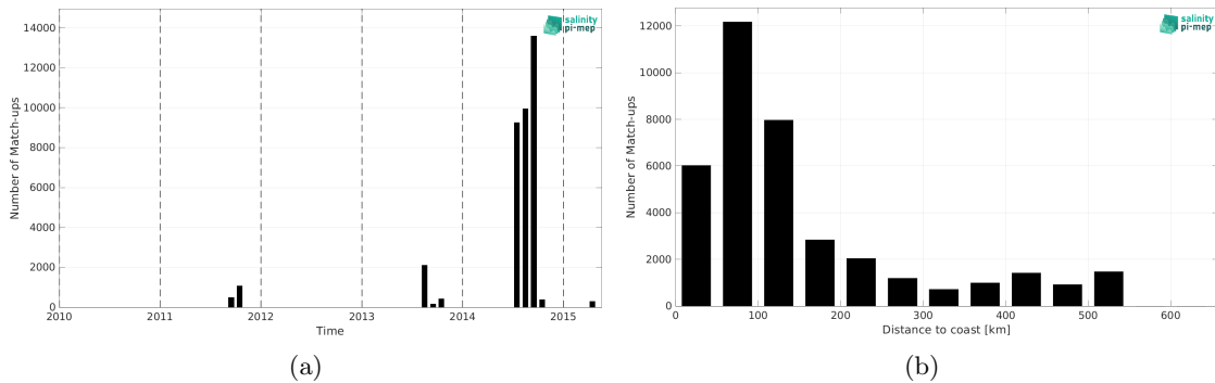
Figure 1: Number of match-ups between TSG (Amundsen) and Aquarius SSS L3 OR v5 - 7-Day running (NASA-GSFC) SSS as a function of time (a) and as function of the distance to coast (b) over the Global Ocean Pi-MEP region and for the full satellite product period.
