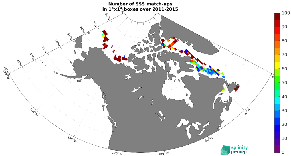
Figure 4: Number of SSS match-ups between TSG (Amundsen) SSS and the Aquarius SSS L3 OR v5 - 7-Day running (NASA-GSFC) SSS product for the Global Ocean Pi-MEP region over 1^\circ \times 1^\circ boxes and for the full satellite product period.
