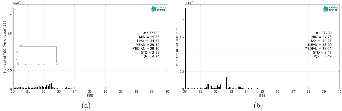
Figure 2: Histograms of SSS from TSG (Amundsen) (a) and Aquarius SSS L3 OR v5 - 7-Day running (NASA-GSFC) (b) considering all match-up pairs per bins of 0.1 over the Global Ocean Pi-MEP region and for the full satellite product period.
