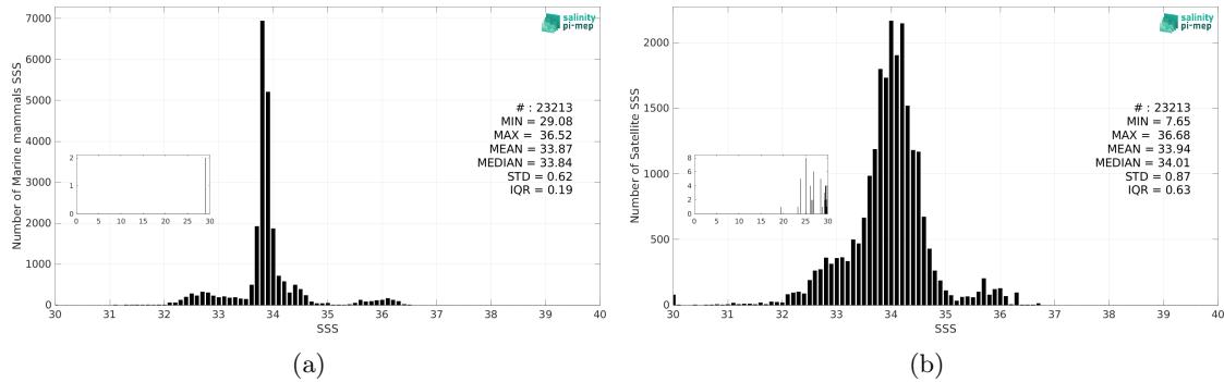
Figure 3: Histograms of SSS from Marine mammals (a) and Aquarius SSS L3 OR v5 - 7-Day running (NASA-GSFC) (b) considering all match-up pairs per bins of 0.1 over the Global Ocean Pi-MEP region and for the full satellite product period.
