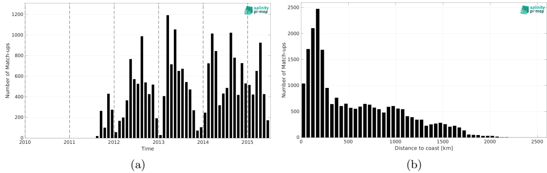
Figure 2: Number of match-ups between Marine mammals and Aquarius SSS L3 OR v5 - 7-Day running (NASA-GSFC) SSS as a function of time (a) and as function of the distance to coast (b) over the Global Ocean Pi-MEP region and for the full satellite product period.
