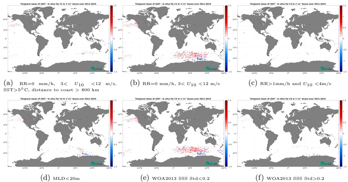
Figure 14: Temporal mean gridded over spatial boxes of size 1^\circ \times 1^\circ of \Delta\text{SSS} (Aquarius SSS L3 OR v5 - 7-Day running (NASA-GSFC) - Marine mammals) for 6 different subdatasets corresponding to:RR=0 mm/h, 3 < U_{10} < 12 m/s, SST>5°C, distance to coast > 800 km (a), RR=0 mm/h, 3 < U_{10} < 12 m/s (b), RR>1mm/h and U_{10} < 4 m/s (c),MLD<20m (d),WOA2013 SSS Std<0.2 (e),WOA2013 SSS Std>0.2 (f).
