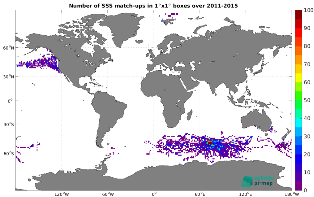
Figure 5: Number of SSS match-ups between Marine mammals SSS and the Aquarius SSS L3 OR v5 - 7-Day running (NASA-GSFC) SSS product for the Global Ocean Pi-MEP region over 1^\circ \times 1^\circ boxes and for the full satellite product period.
