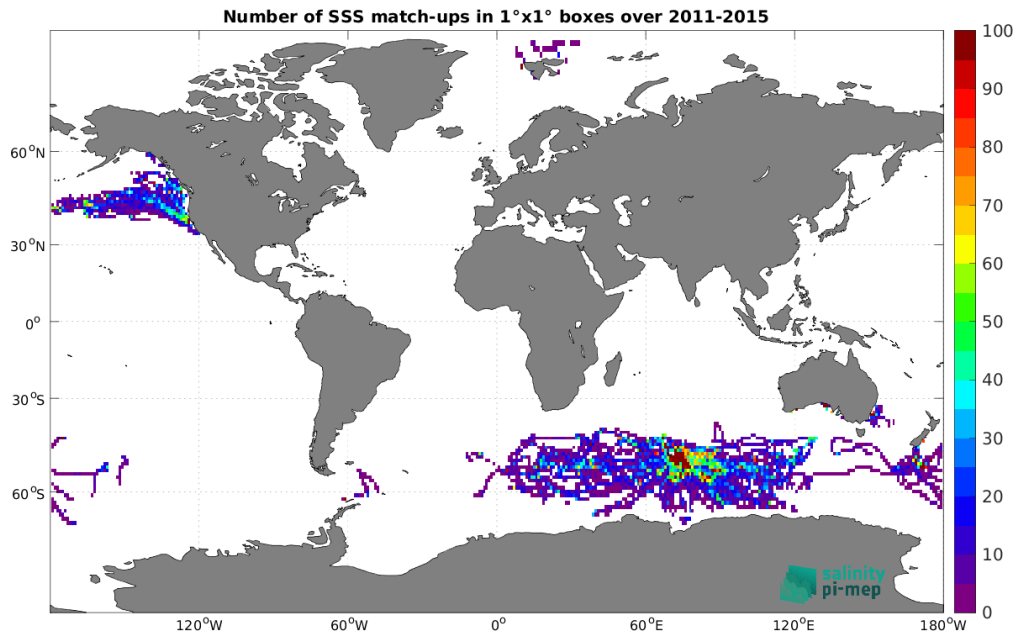
Figure 4: Number of SSS match-ups between Marine mammals SSS and the Aquarius SSS L3 OR v5 - 7-Day running (NASA-GSFC) SSS product for the Global Ocean Pi-MEP region over 1^\circ \times 1^\circ boxes and for the full satellite product period.
