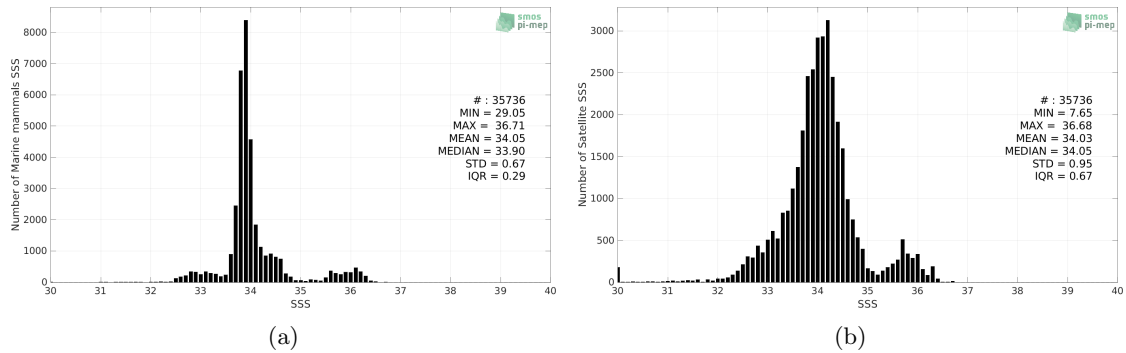
Figure 2: Histograms of SSS from Marine mammals (a) and Aquarius SSS L3 OR v5 - 7-Day running (NASA-GSFC) (b) considering all match-up pairs per bins of 0.1 over the Global Ocean Pi-MEP region and for the full satellite product period.
