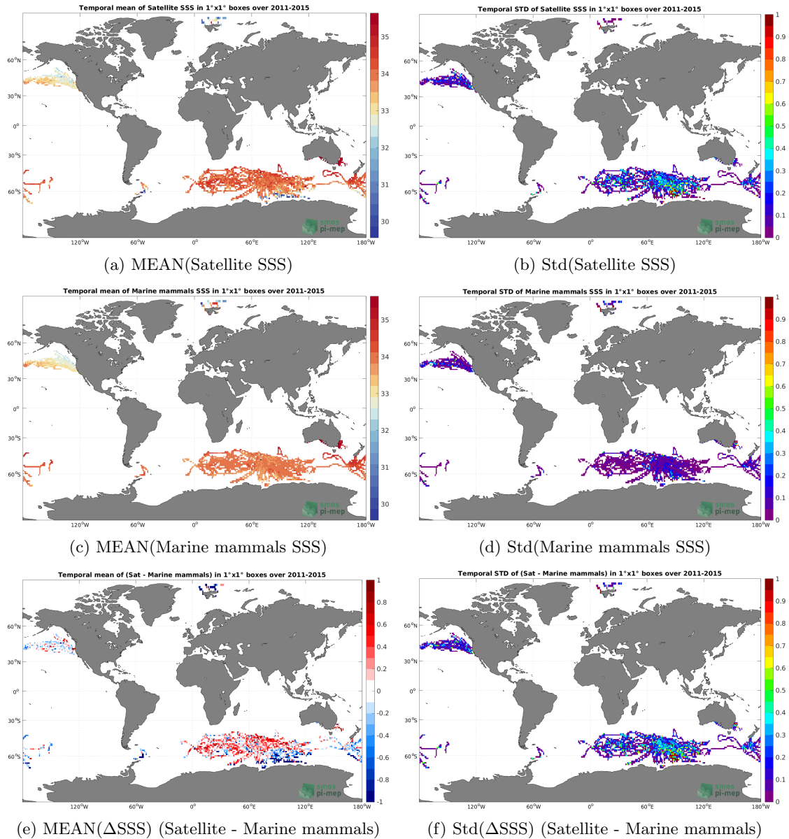
Figure 6: Temporal mean (left) and Std (right) of SSS from Aquarius SSS L3 OR v5 - 7-Day running (NASA-GSFC) (top), Marine mammals (middle), and of \Delta SSS (Satellite - Marine mammals). Only match-up pairs are used to generate these maps.
