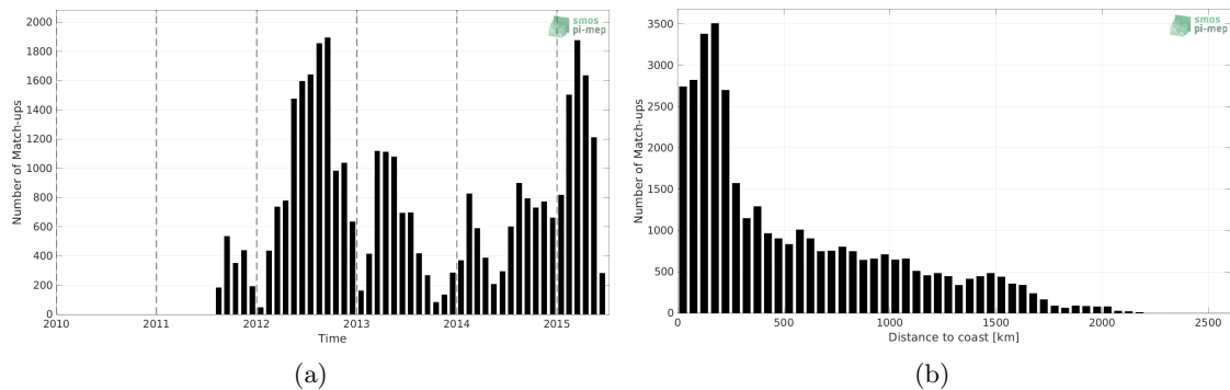
Figure 1: Number of match-ups between Marine mammals and Aquarius SSS L3 OR v5 - 7-Day running (NASA-GSFC) SSS as a function of time (a) and as function of the distance to coast (b) over the Global Ocean Pi-MEP region and for the full satellite product period.
