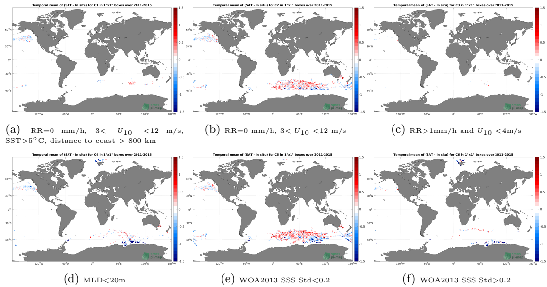
Figure 12: Temporal mean gridded over spatial boxes of size 1^\circ \times 1^\circ of \Delta SSS (Aquarius SSS L3 OR v5 - 7-Day running (NASA-GSFC) - Marine mammals) for 6 different subdatasets corresponding to:RR=0 mm/h, 3 < U_{10} < 12 m/s, SST >5^\circ\text{C} , distance to coast > 800 km (a), RR=0 mm/h, 3 < U_{10} < 12 m/s (b), RR >1 mm/h and U_{10} < 4 m/s (c),MLD <20 m (d),WOA2013 SSS Std <0.2 (e),WOA2013 SSS Std >0.2 (f).
