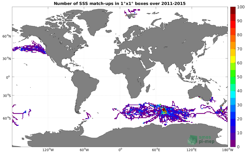
Figure 4: Number of SSS match-ups between Marine mammals SSS and the Aquarius SSS L3 OR v5 - 7-Day running (NASA-GSFC) SSS product for the Global Ocean Pi-MEP region over 1° × 1° boxes and for the full satellite product period.
