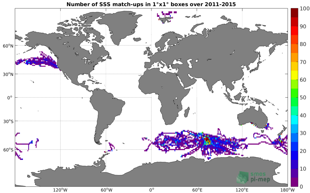
Figure 4: Number of SSS match-ups between Marine mammals SSS and the Aquarius SSS L3 OR v5 - 7-Day running (NASA-GSFC) SSS product for the Global Ocean Pi-MEP region over 1°×1° boxes and for the full satellite product period.
