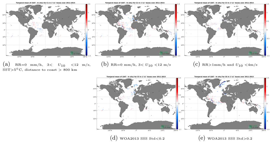
Figure 11: Temporal mean gridded over spatial boxes of size 1^\circ \times 1^\circ of \Delta\text{SSS} (Aquarius SSS L3 OR v5 - 7-Day running (NASA-GSFC) - Surface drifters) for 5 different subdatasets corresponding to:RR=0 mm/h, 3 < U_{10} < 12 m/s, SST >5^\circ\text{C} , distance to coast > 800 km (a), RR=0 mm/h, 3 < U_{10} < 12 m/s (b), RR >1 mm/h and U_{10} < 4 m/s (c), WOA2013 SSS Std <0.2 (d), WOA2013 SSS Std >0.2 (e).
