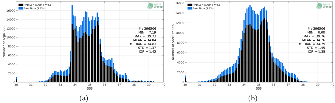
Figure 2: Histograms of SSS from Argo (a) and Aquarius-L3-OR-V5-7DAY-RUNNING-1DEG (b) considering all match-up pairs per bins of 0.1 over the Global Ocean Pi-MEP region and for the full satellite product period.
