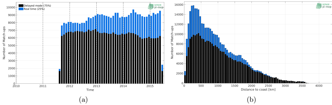
Figure 1: Number of match-ups between Argo and Aquarius-L3-OR-V5-7DAY-RUNNING-1DEG SSS as a function of time (a) and as function of the distance to coast (b) over the Global Ocean Pi-MEP region and for the full satellite product period.
