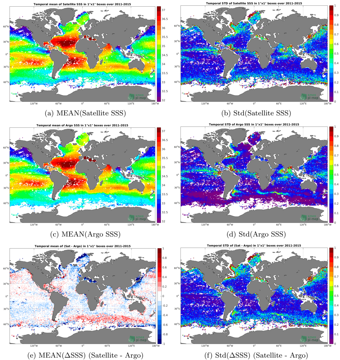
Figure 6: Temporal mean (left) and Std (right) of SSS from Aquarius-L3-OR-V5-7DAY-RUNNING-1DEG (top), Argo (middle), and of \Delta SSS (Satellite - Argo). Only match-up pairs are used to generate these maps.
