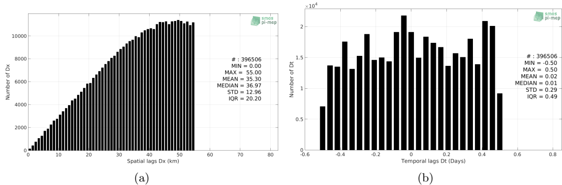
Figure 5: Histograms of the spatial (a) and temporal (b) lags between the time of the Argo measurements and the date of the corresponding Aquarius-L3-OR-V5-7DAY-RUNNING-1DEG SSS product.
