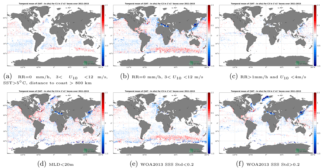
Figure 12: Temporal mean gridded over spatial boxes of size 1^\circ \times 1^\circ of \Delta SSS (Aquarius-L3-OR-V5-7DAY-RUNNING-1DEG - Argo) for 6 different subdatasets corresponding to:RR=0 mm/h, 3 < U_{10} < 12 m/s, SST >5^\circ C, distance to coast > 800 km (a), RR=0 mm/h, 3 < U_{10} < 12 m/s (b), RR >1 mm/h and U_{10} < 4 m/s (c),MLD <20 m (d),WOA2013 SSS Std <0.2 (e),WOA2013 SSS Std >0.2 (f).
