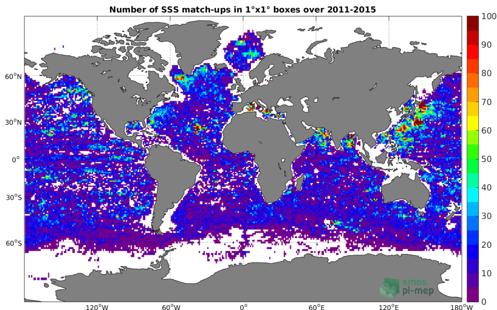
Figure 4: Number of SSS match-ups between Argo SSS and the Aquarius-L3-OR-V5-7DAY-RUNNING-1DEG SSS product for the Global Ocean Pi-MEP region over 1^\circ \times 1^\circ boxes and for the full satellite product period.
