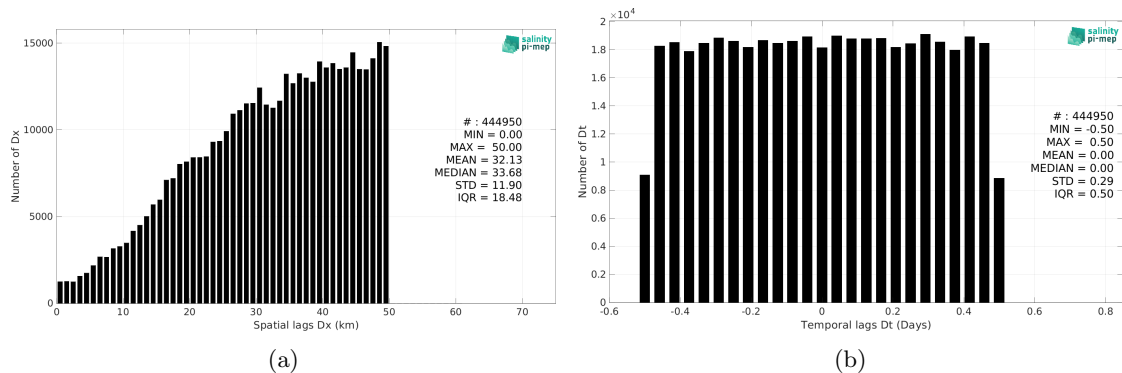
Figure 6: Histograms of the spatial (a) and temporal (b) lags between the location/time of the TSG (SAMOS) measurement and the date of the corresponding Aquarius SSS L3 OR v5 - 7-Day running - Rain mask (NASA-GSFC) SSS pixel.
