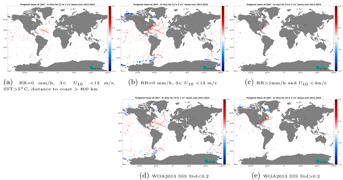
Figure 14: Temporal mean gridded over spatial boxes of size 1^\circ \times 1^\circ of \Delta SSS (Aquarius SSS L3 OR v5 - 7-Day running - Rain mask (NASA-GSFC) - TSG (SAMOS)) for 5 different subdatasets corresponding to:RR=0 mm/h, 3 < U_{10} < 12 m/s, SST > 5^\circ\text{C} , distance to coast > 800 km (a), RR=0 mm/h, 3 < U_{10} < 12 m/s (b), RR > 1 mm/h and U_{10} < 4 m/s (c), WOA2013 SSS Std < 0.2 (d), WOA2013 SSS Std > 0.2 (e).
