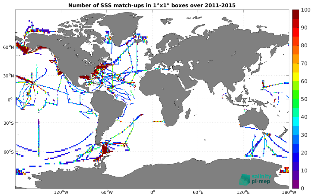
Figure 5: Number of SSS match-ups between TSG (SAMOS) SSS and the Aquarius SSS L3 OR v5 - 7-Day running - Rain mask (NASA-GSFC) SSS product for the Global Ocean Pi-MEP region over 1^\circ \times 1^\circ boxes and for the full satellite product period.
