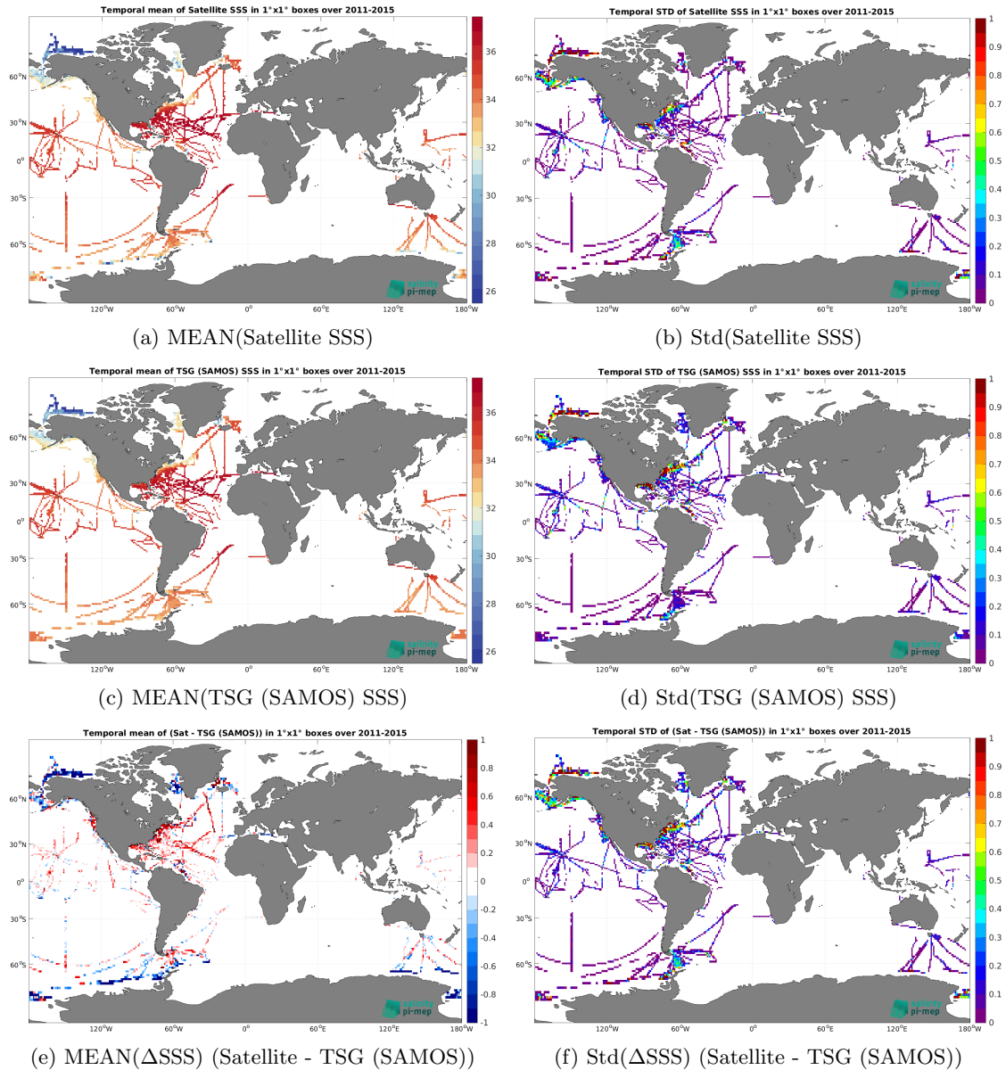
Figure 7: Temporal mean (left) and Std (right) of SSS from Aquarius SSS L3 OR v5 - 7-Day running - Rain mask (NASA-GSFC) (top), TSG (SAMOS) (middle), and of \Delta SSS (Satellite - TSG (SAMOS)). Only match-up pairs are used to generate these maps.
