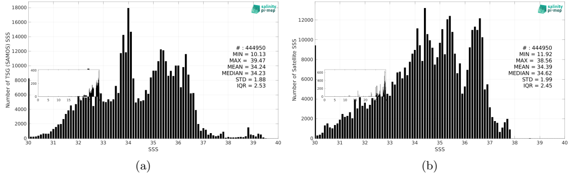
Figure 3: Histograms of SSS from TSG (SAMOS) (a) and Aquarius SSS L3 OR v5 - 7-Day running - Rain mask (NASA-GSFC) (b) considering all match-up pairs per bins of 0.1 over the Global Ocean Pi-MEP region and for the full satellite product period.
