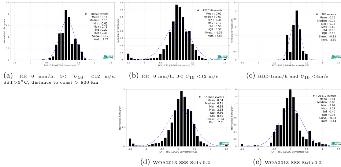
Figure 15: Normalized histogram of \Delta SSS (Aquarius SSS L3 OR v5 - 7-Day running - Rain mask (NASA-GSFC) - TSG (LEGOS-Survostral)) for 5 different subdatasets corresponding to: RR=0 mm/h, 3 < U_{10} < 12 m/s, SST>5°C, distance to coast > 800 km (a), RR=0 mm/h, 3 < U_{10} < 12 m/s (b), RR>1mm/h and U_{10} < 4 m/s (c), WOA2013 SSS Std<0.2 (d), WOA2013 SSS Std>0.2 (e).
