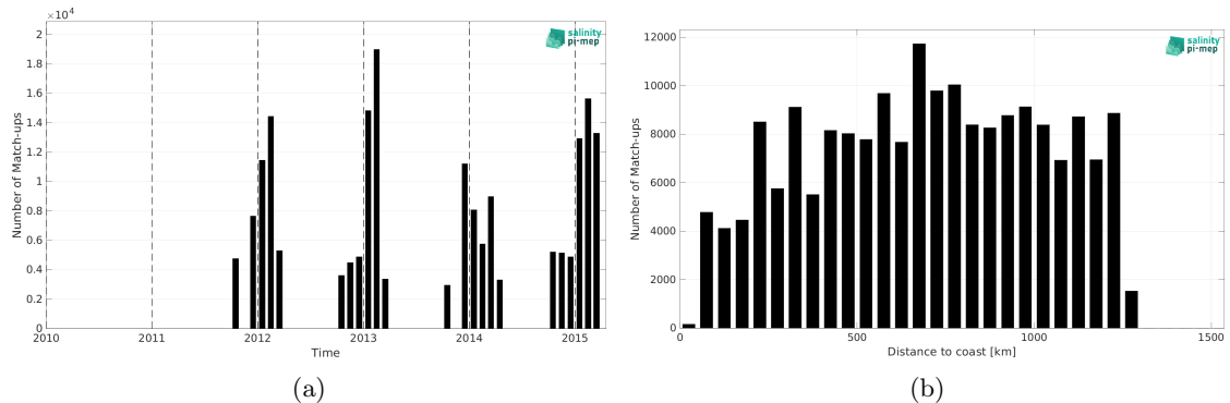
Figure 2: Number of match-ups between TSG (LEGOS-Survostral) and Aquarius SSS L3 OR v5 - 7-Day running - Rain mask (NASA-GSFC) SSS as a function of time (a) and as function of the distance to coast (b) over the Global Ocean Pi-MEP region and for the full satellite product period.
