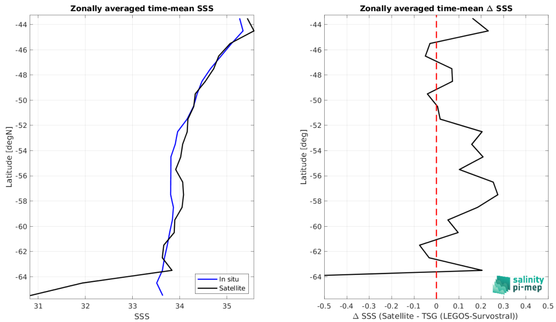
Figure 9: Left panel: Zonal mean SSS from Aquarius SSS L3 OR v5 - 7-Day running - Rain mask (NASA-GSFC) satellite product (black) and from TSG (LEGOS-Survostral) (blue). Right panel: Zonal mean of \Delta SSS (Satellite - TSG (LEGOS-Survostral)) for all the collected Pi-MEP match-up pairs estimated over the full satellite product period.
