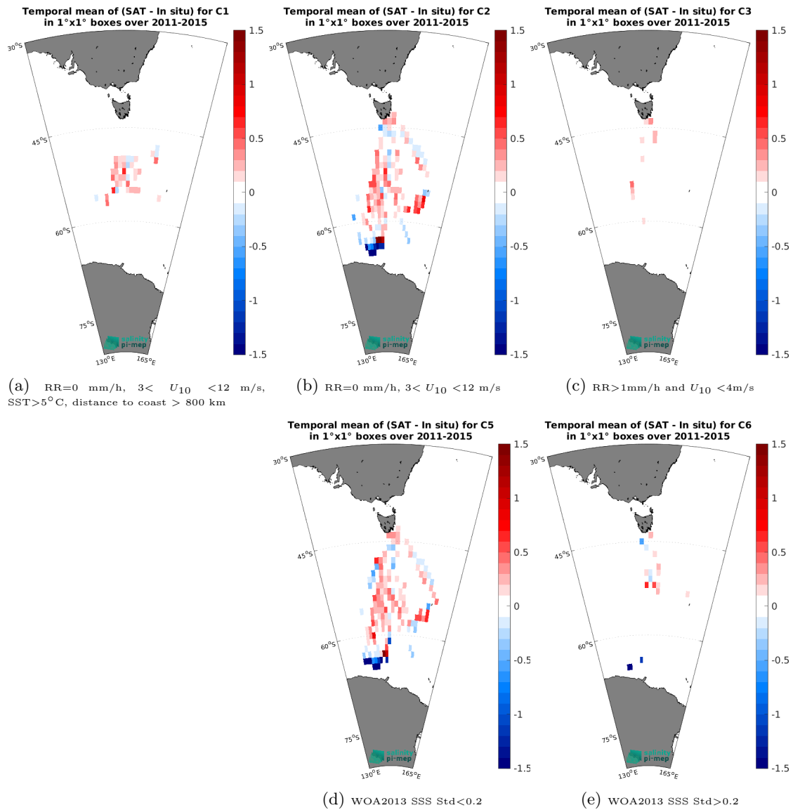
Figure 14: Temporal mean gridded over spatial boxes of size 1^\circ \times 1^\circ of \Delta SSS (Aquarius SSS L3 OR v5 - 7-Day running - Rain mask (NASA-GSFC) - TSG (LEGOS-Survostral)) for 5 different subdatasets corresponding to:RR=0 mm/h, 3 < U_{10} < 12 m/s, SST>5°C, distance to coast > 800 km (a), RR=0 mm/h, 3 < U_{10} < 12 m/s (b), RR>1mm/h and U_{10} < 4 m/s (c), WOA2013 SSS Std<0.2 (d), WOA2013 SSS Std>0.2 (e).
