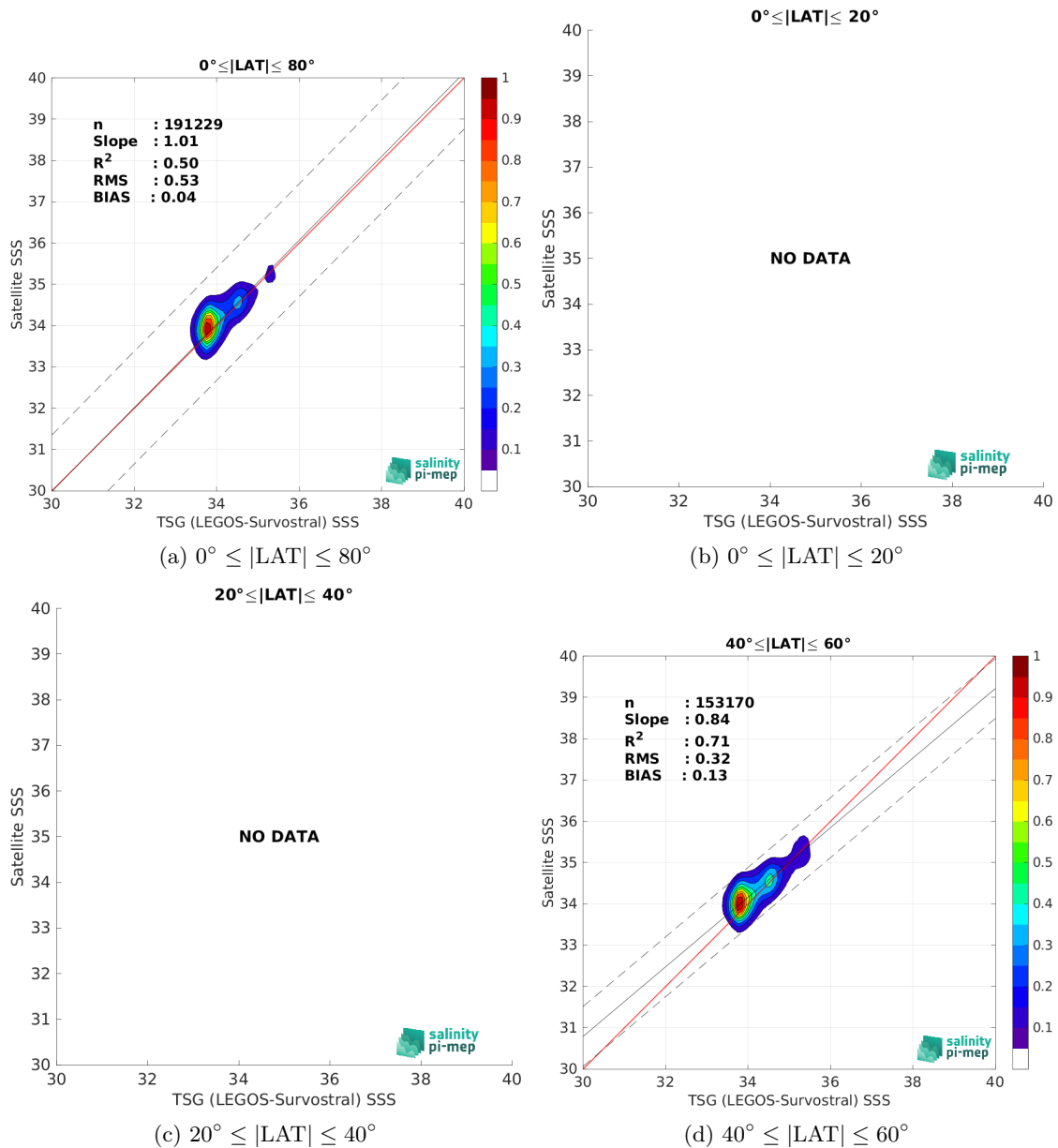
Figure 10: Contour maps of the concentration of Aquarius SSS L3 OR v5 - 7-Day running - Rain mask (NASA-GSFC) SSS (y-axis) versus TSG (LEGOS-Survostral) SSS (x-axis) at match-up pairs for different latitude bands. For each plot, the red line shows x=y . The black thin and dashed lines indicate a linear fit through the data cloud and the \pm 95\% confidence levels, respectively. The number match-up pairs n , the slope and R^2 coefficient of the linear fit, the root mean square (RMS) and the mean bias between satellite and in situ data are indicated for each latitude band in each plots.
