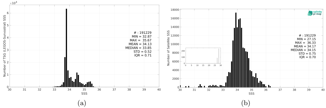
Figure 3: Histograms of SSS from TSG (LEGOS-Survostral) (a) and Aquarius SSS L3 OR v5 - 7-Day running - Rain mask (NASA-GSFC) (b) considering all match-up pairs per bins of 0.1 over the Global Ocean Pi-MEP region and for the full satellite product period.
