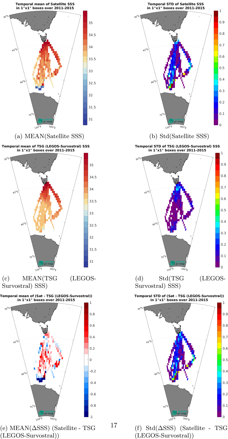
Figure 7: Temporal mean (left) and Std (right) of SSS from Aquarius SSS L3 OR v5 - 7-Day running - Rain mask (NASA-GSFC) (top), TSG (LEGOS-Survostral) (middle), and of \Delta SSS (Satellite - TSG (LEGOS-Survostral)). Only match-up pairs are used to generate these maps.
