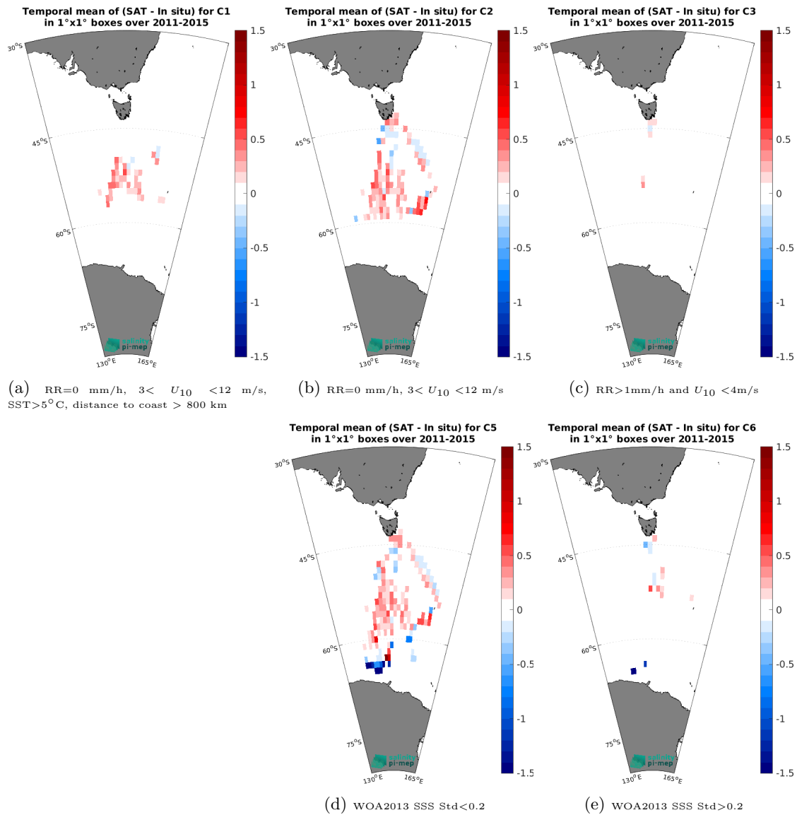
Figure 12: Temporal mean gridded over spatial boxes of size 1^\circ \times 1^\circ of \Delta\text{SSS} (Aquarius SSS L3 OR v5 - 7-Day running - Rain mask (NASA-GSFC) - TSG (LEGOS-Survostral)) for 5 different subdatasets corresponding to: RR=0 mm/h, 3 < U_{10} < 12 m/s, SST > 5^\circ\text{C} , distance to coast > 800 km (a), RR=0 mm/h, 3 < U_{10} < 12 m/s (b), RR > 1 mm/h and U_{10} < 4 m/s (c), WOA2013 SSS Std < 0.2 (d), WOA2013 SSS Std > 0.2 (e).
