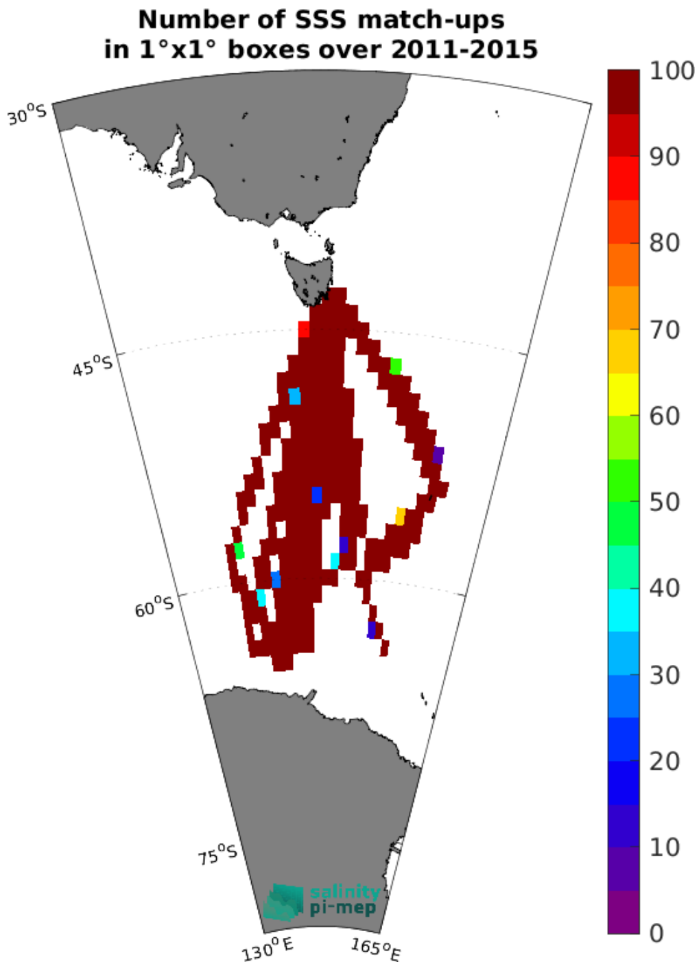
Figure 4: Number of SSS match-ups between TSG (LEGOS-Survostral) SSS and the Aquarius SSS L3 OR v5 - 7-Day running - Rain mask (NASA-GSFC) SSS product for the Global Ocean Pi-MEP region over 1°x1° boxes and for the full satellite product period.
