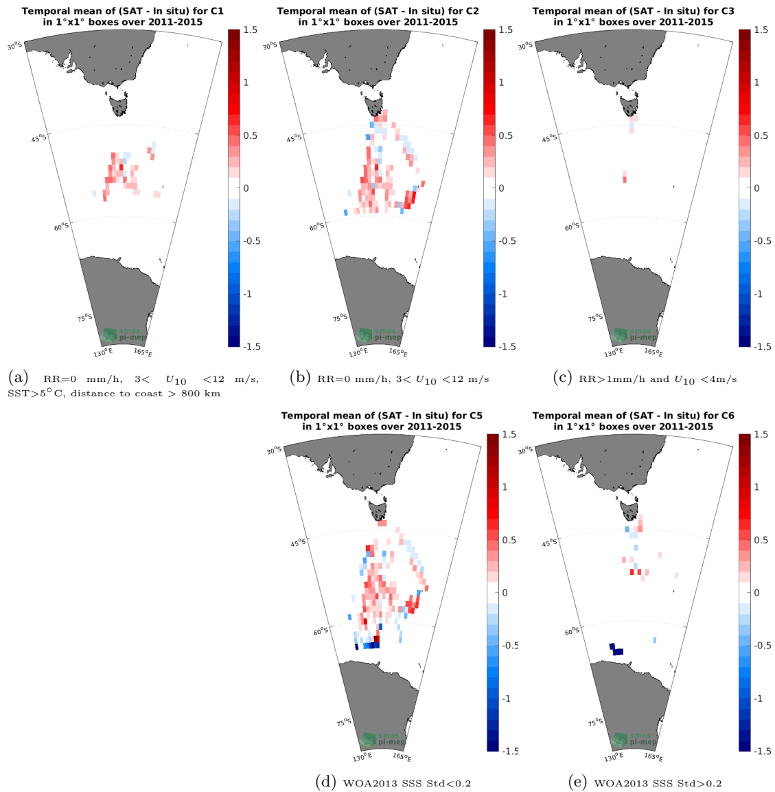
Figure 12: Temporal mean gridded over spatial boxes of size 1^\circ \times 1^\circ of \Delta SSS (Aquarius SSS L3 OR v5 - 7-Day running - Rain mask (NASA-GSFC) - TSG (LEGOS-Survostral)) for 5 different subdatasets corresponding to:RR=0 mm/h, 3 < U_{10} < 12 m/s, SST>5°C, distance to coast > 800 km (a), RR=0 mm/h, 3 < U_{10} < 12 m/s (b), RR>1mm/h and U_{10} < 4 m/s (c), WOA2013 SSS Std<0.2 (d), WOA2013 SSS Std>0.2 (e).
