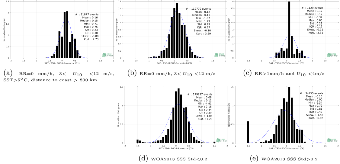
Figure 13: Normalized histogram of \Delta SSS (Aquarius-L3-OR-V5-7DAY-RUNNING-RAIN-MASK-1DEG - TSG-LEGOS-Survostral) for 5 different subdatasets corresponding to: RR=0 mm/h, 3 < U_{10} < 12 m/s, SST > 5°C, distance to coast > 800 km (a), RR=0 mm/h, 3 < U_{10} < 12 m/s (b), RR > 1mm/h and U_{10} < 4 m/s (c), WOA2013 SSS Std < 0.2 (d), WOA2013 SSS Std > 0.2 (e).
