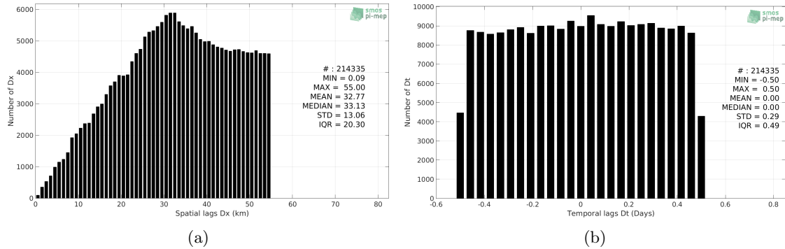
Figure 5: Histograms of the spatial (a) and temporal (b) lags between the time of the TSG-LEGOS-Survostral measurements and the date of the corresponding Aquarius-L3-OR-V5-7DAY-RUNNING-RAIN-MASK-1DEG SSS product.
