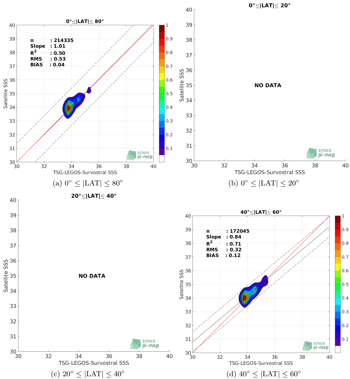
Figure 9: Contour maps of the concentration of Aquarius-L3-OR-V5-7DAY-RUNNING-RAIN-MASK-1DEG SSS (y-axis) versus TSG-LEGOS-Survostral SSS (x-axis) at match-up pairs for different latitude bands. For each plot, the red line shows x=y . The black thin and dashed lines indicate a linear fit through the data cloud and the \pm 95\% confidence levels, respectively. The number match-up pairs n , the slope and R^2 coefficient of the linear fit, the root mean square (RMS) and the mean bias between satellite and in situ data are indicated for each latitude band in each plots.
