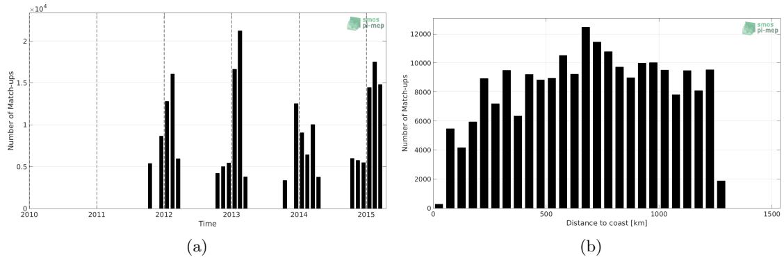
Figure 1: Number of match-ups between TSG-LEGOS-Survostral and Aquarius-L3-OR-V5-7DAY-RUNNING-RAIN-MASK-1DEG SSS as a function of time (a) and as function of the distance to coast (b) over the Global Ocean Pi-MEP region and for the full satellite product period.
