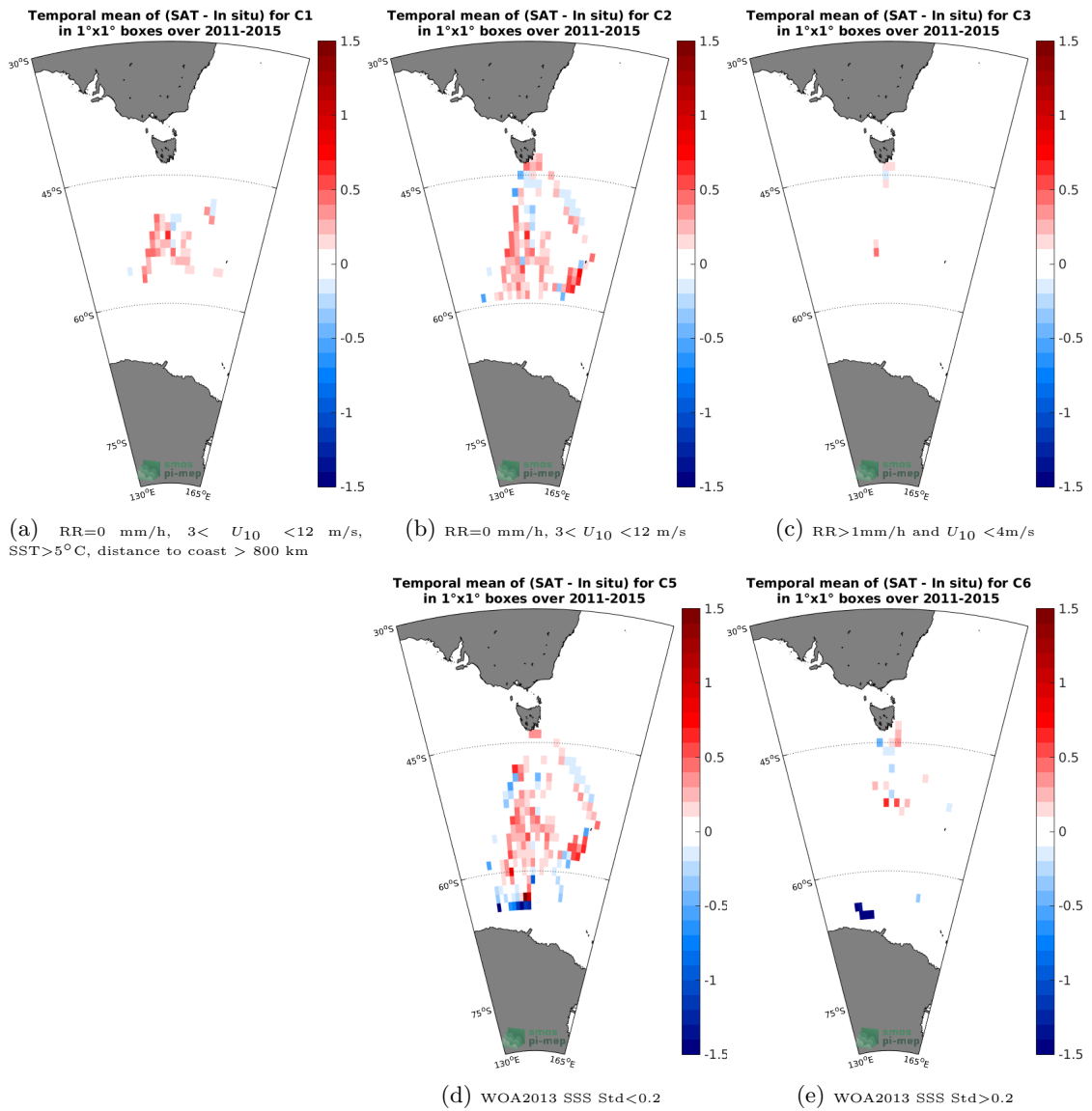
Figure 12: Temporal mean gridded over spatial boxes of size 1°x1° of \Delta SSS (Aquarius-L3-OR-V5-7DAY-RUNNING-RAIN-MASK-1DEG - TSG-LEGOS-Survostral) for 5 different subdatasets corresponding to: RR=0 mm/h, 3 < U_{10} < 12 m/s, SST > 5°C, distance to coast > 800 km (a), RR=0 mm/h, 3 < U_{10} < 12 m/s (b), RR > 1mm/h and U_{10} < 4 m/s (c), WOA2013 SSS Std < 0.2 (d), WOA2013 SSS Std > 0.2 (e).
