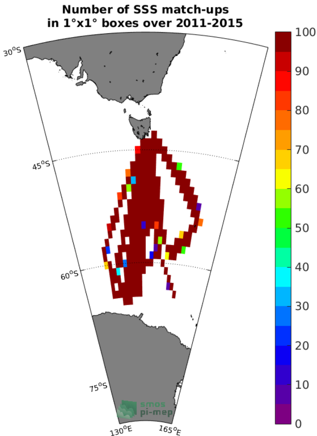
Figure 4: Number of SSS match-ups between TSG-LEGOS-Survostral SSS and the Aquarius-L3-OR-V5-7DAY-RUNNING-RAIN-MASK-1DEG SSS product for the Global Ocean Pi-MEP region over 1°x1° boxes and for the full satellite product period.
