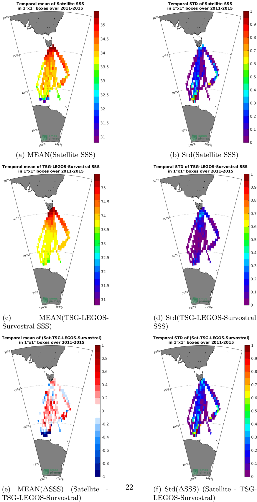
Figure 6: Temporal mean (left) and Std (right) of SSS from Aquarius-L3-OR-V5-7DAY-RUNNING-RAIN-MASK-1DEG (top), TSG-LEGOS-Survostral (middle), and of \Delta SSS (Satellite - TSG-LEGOS-Survostral). Only match-up pairs are used to generate these maps.
