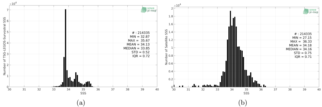
Figure 2: Histograms of SSS from TSG-LEGOS-Survostral (a) and Aquarius-L3-OR-V5-7DAY-RUNNING-RAIN-MASK-1DEG (b) considering all match-up pairs per bins of 0.1 over the Global Ocean Pi-MEP region and for the full satellite product period.
