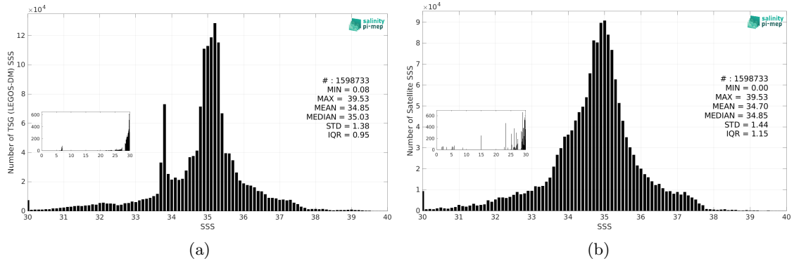
Figure 3: Histograms of SSS from TSG (LEGOS-DM) (a) and Aquarius SSS L3 OR v5 - 7-Day running - Rain mask (NASA-GSFC) (b) considering all match-up pairs per bins of 0.1 over the Global Ocean Pi-MEP region and for the full satellite product period.
