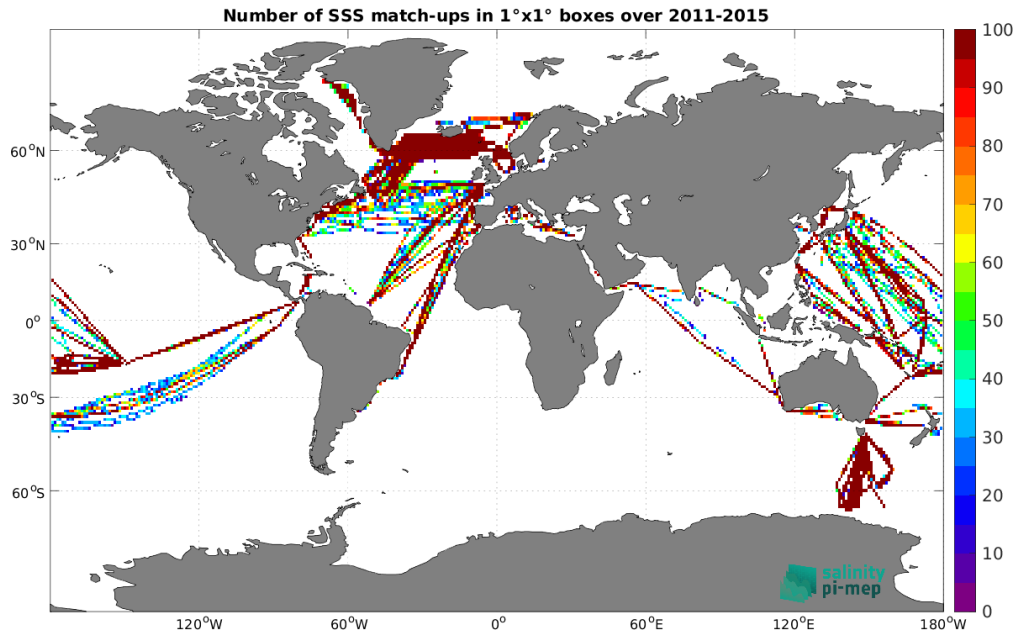
Figure 5: Number of SSS match-ups between TSG (LEGOS-DM) SSS and the Aquarius SSS L3 OR v5 - 7-Day running - Rain mask (NASA-GSFC) SSS product for the Global Ocean Pi-MEP region over 1^\circ \times 1^\circ boxes and for the full satellite product period.
