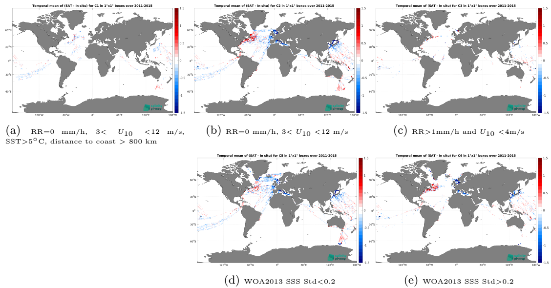
Figure 12: Temporal mean gridded over spatial boxes of size 1^\circ \times 1^\circ of \Delta\text{SSS} (Aquarius SSS L3 OR v5 - 7-Day running - Rain mask (NASA-GSFC) - TSG (LEGOS-DM)) for 5 different subdatasets corresponding to:RR=0 mm/h, 3 < U_{10} < 12 m/s, SST > 5^\circ\text{C} , distance to coast > 800 km (a), RR=0 mm/h, 3 < U_{10} < 12 m/s (b), RR > 1 mm/h and U_{10} < 4 m/s (c), WOA2013 SSS Std < 0.2 (d), WOA2013 SSS Std > 0.2 (e).
