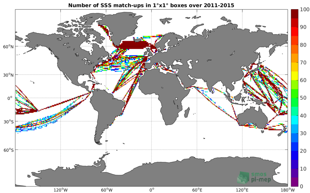
Figure 4: Number of SSS match-ups between TSG-LEGOS-DM SSS and the Aquarius-L3-OR-V5-7DAY-RUNNING-RAIN-MASK-1DEG SSS product for the Global Ocean Pi-MEP region over 1°x1° boxes and for the full satellite product period.
