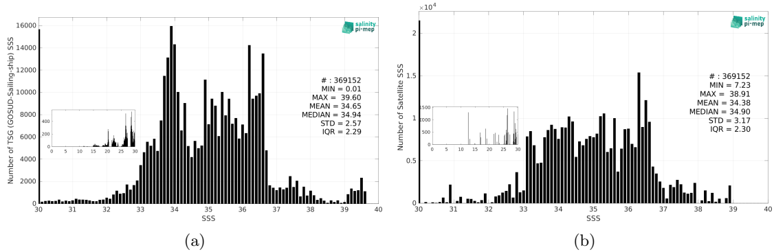
Figure 3: Histograms of SSS from TSG (GOSUD-Sailing-ship) (a) and Aquarius SSS L3 OR v5 - 7-Day running - Rain mask (NASA-GSFC) (b) considering all match-up pairs per bins of 0.1 over the Global Ocean Pi-MEP region and for the full satellite product period.
