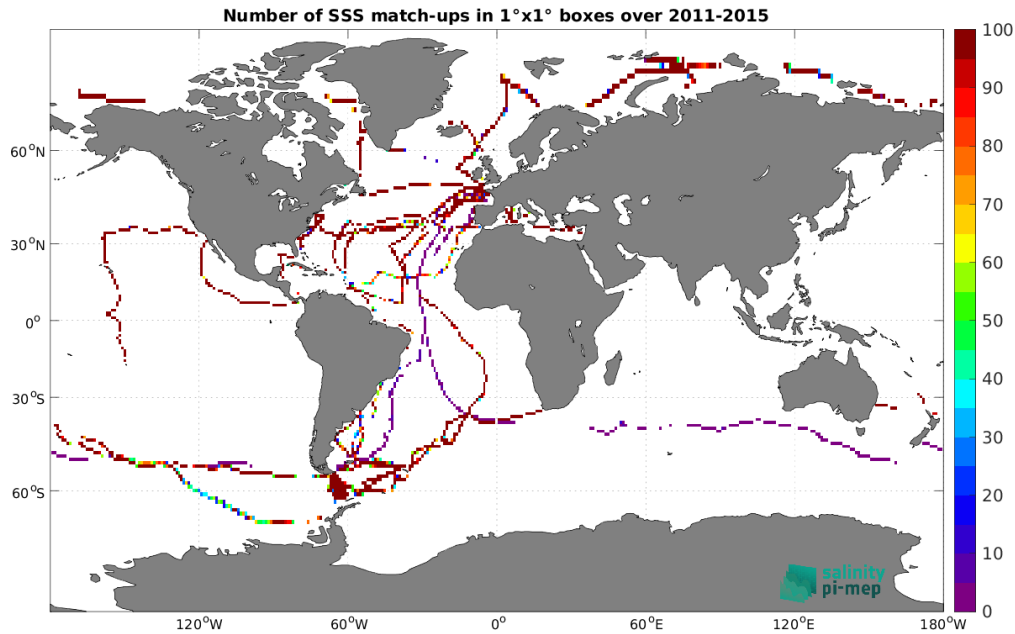
Figure 5: Number of SSS match-ups between TSG (GOSUD-Sailing-ship) SSS and the Aquarius SSS L3 OR v5 - 7-Day running - Rain mask (NASA-GSFC) SSS product for the Global Ocean Pi-MEP region over 1^\circ \times 1^\circ boxes and for the full satellite product period.
