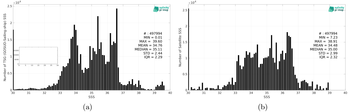
Figure 2: Histograms of SSS from TSG (GOSUD-Sailing-ship) (a) and Aquarius SSS L3 OR v5 - 7-Day running - Rain mask (NASA-GSFC) (b) considering all match-up pairs per bins of 0.1 over the Global Ocean Pi-MEP region and for the full satellite product period.
