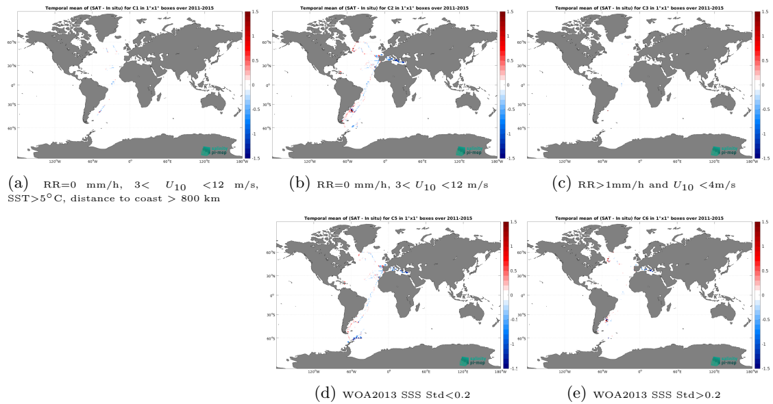
Figure 12: Temporal mean gridded over spatial boxes of size 1^\circ \times 1^\circ of \Delta\text{SSS} (Aquarius SSS L3 OR v5 - 7-Day running - Rain mask (NASA-GSFC) - TSG (CSIC-UTM)) for 5 different subdatasets corresponding to:RR=0 mm/h, 3 < U_{10} < 12 m/s, SST > 5^\circ\text{C} , distance to coast > 800 km (a), RR=0 mm/h, 3 < U_{10} < 12 m/s (b), RR > 1\text{mm/h} and U_{10} < 4\text{m/s} (c), WOA2013 SSS Std < 0.2 (d), WOA2013 SSS Std > 0.2 (e).
