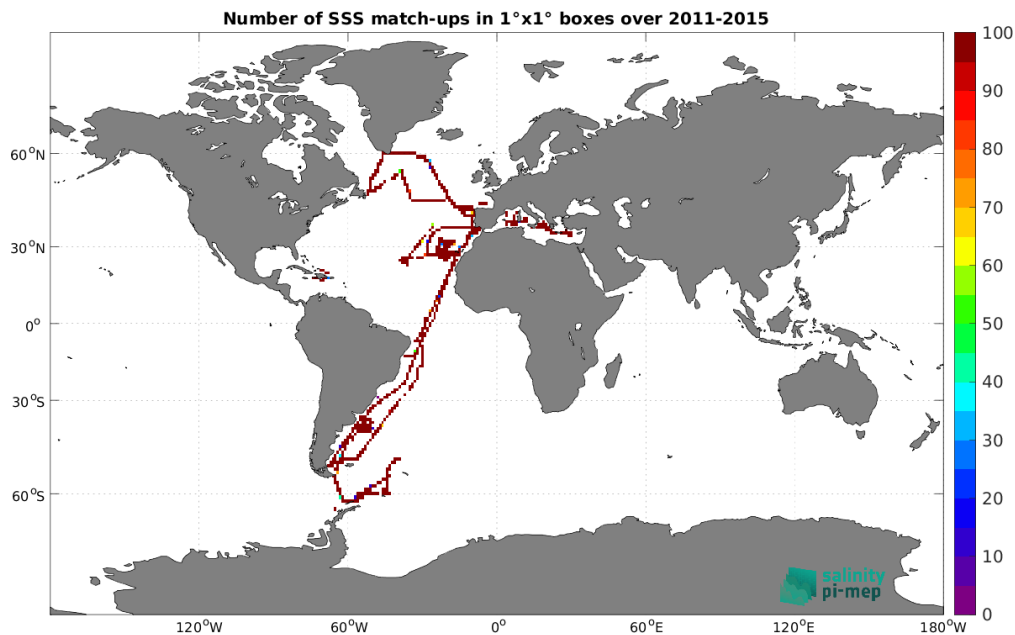
Figure 4: Number of SSS match-ups between TSG (CSIC-UTM) SSS and the Aquarius SSS L3 OR v5 - 7-Day running - Rain mask (NASA-GSFC) SSS product for the Global Ocean Pi-MEP region over 1^\circ \times 1^\circ boxes and for the full satellite product period.
