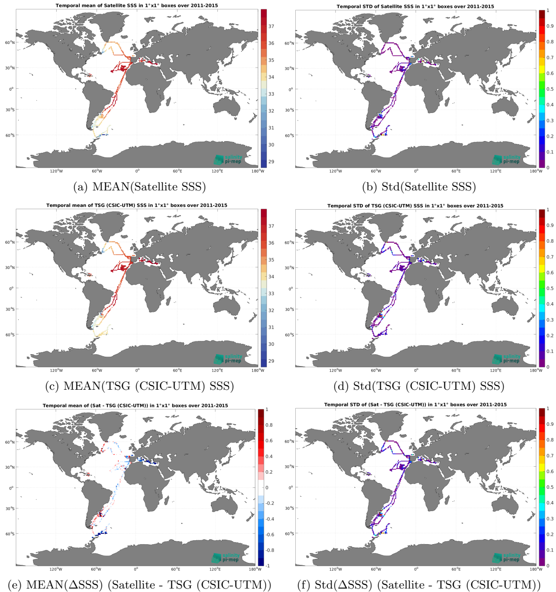
Figure 6: Temporal mean (left) and Std (right) of SSS from Aquarius SSS L3 OR v5 - 7-Day running - Rain mask (NASA-GSFC) (top), TSG (CSIC-UTM) (middle), and of \Delta SSS (Satellite - TSG (CSIC-UTM)). Only match-up pairs are used to generate these maps.
