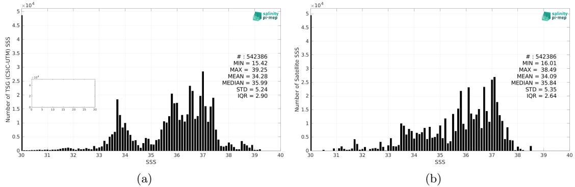
Figure 2: Histograms of SSS from TSG (CSIC-UTM) (a) and Aquarius SSS L3 OR v5 - 7-Day running - Rain mask (NASA-GSFC) (b) considering all match-up pairs per bins of 0.1 over the Global Ocean Pi-MEP region and for the full satellite product period.
