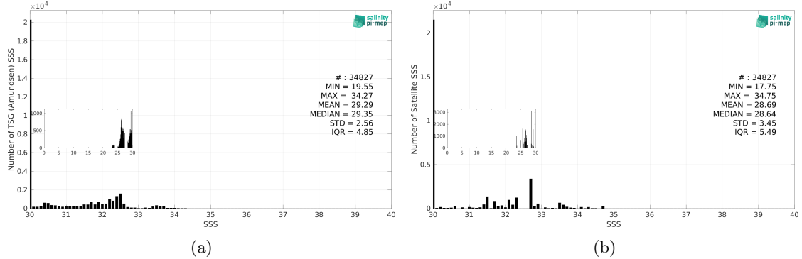
Figure 3: Histograms of SSS from TSG (Amundsen) (a) and Aquarius SSS L3 OR v5 - 7-Day running - Rain mask (NASA-GSFC) (b) considering all match-up pairs per bins of 0.1 over the Global Ocean Pi-MEP region and for the full satellite product period.
