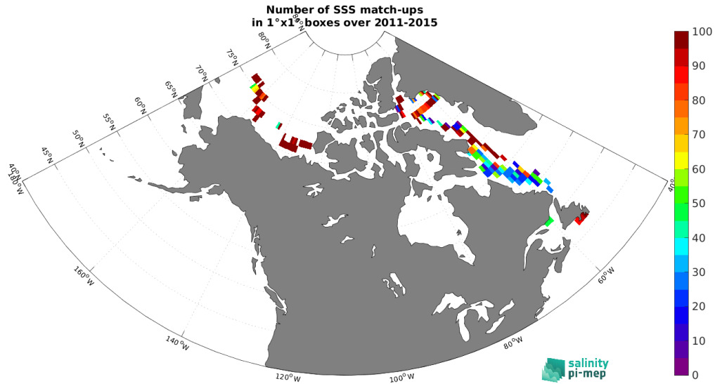
Figure 5: Number of SSS match-ups between TSG (Amundsen) SSS and the Aquarius SSS L3 OR v5 - 7-Day running - Rain mask (NASA-GSFC) SSS product for the Global Ocean Pi-MEP region over 1^\circ \times 1^\circ boxes and for the full satellite product period.
