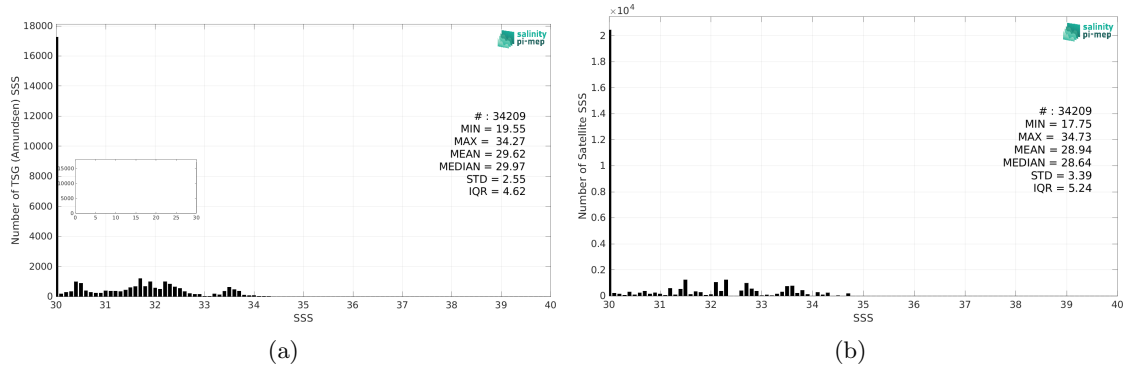
Figure 2: Histograms of SSS from TSG (Amundsen) (a) and Aquarius SSS L3 OR v5 - 7-Day running - Rain mask (NASA-GSFC) (b) considering all match-up pairs per bins of 0.1 over the Global Ocean Pi-MEP region and for the full satellite product period.
