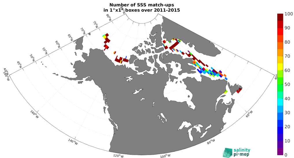
Figure 4: Number of SSS match-ups between TSG (Amundsen) SSS and the Aquarius SSS L3 OR v5 - 7-Day running - Rain mask (NASA-GSFC) SSS product for the Global Ocean Pi-MEP region over 1°×1° boxes and for the full satellite product period.
