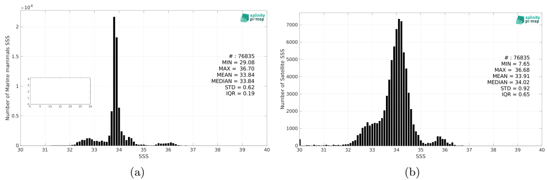
Figure 2: Histograms of SSS from Marine mammals (a) and Aquarius SSS L3 OR v5 - 7-Day running - Rain mask (NASA-GSFC) (b) considering all match-up pairs per bins of 0.1 over the Global Ocean Pi-MEP region and for the full satellite product period.
