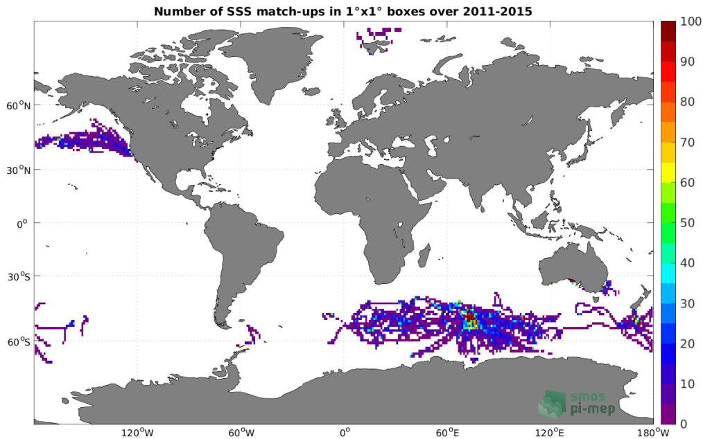
Figure 4: Number of SSS match-ups between Marine mammals SSS and the Aquarius SSS L3 OR v5 - 7-Day running - Rain mask (NASA-GSFC) SSS product for the Global Ocean Pi-MEP region over 1^\circ \times 1^\circ boxes and for the full satellite product period.
