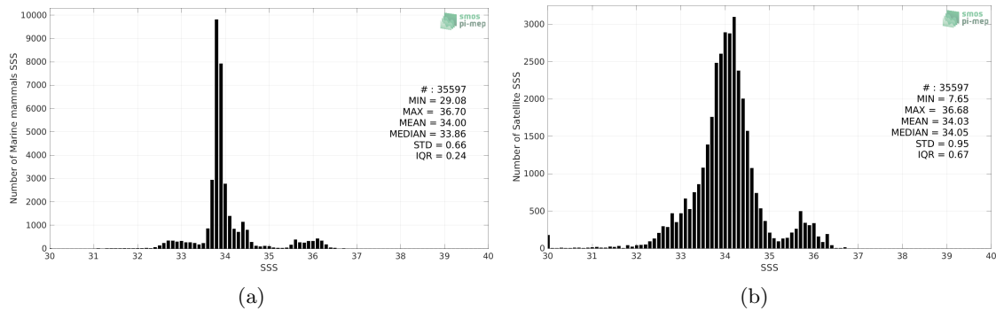
Figure 2: Histograms of SSS from Marine mammals (a) and Aquarius SSS L3 OR v5 - 7-Day running - Rain mask (NASA-GSFC) (b) considering all match-up pairs per bins of 0.1 over the Global Ocean Pi-MEP region and for the full satellite product period.
