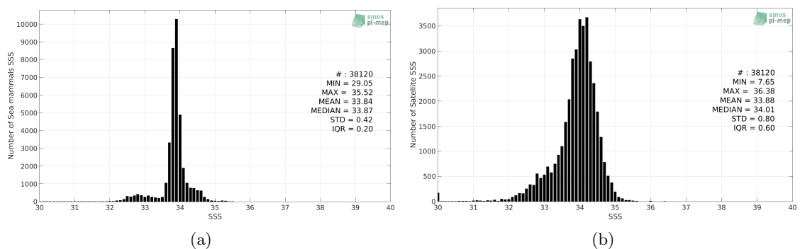
Figure 2: Histograms of SSS from Sea mammals (a) and Aquarius-L3-OR-V5-7DAY-RUNNING-RAIN-MASK-1DEG (b) considering all match-up pairs per bins of 0.1 over the Global Ocean Pi-MEP region and for the full satellite product period.
