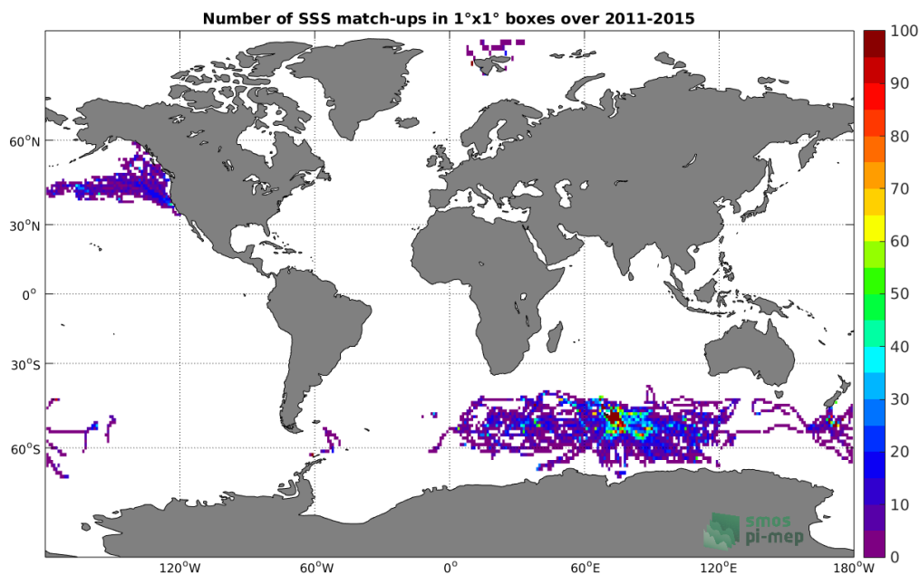
Figure 4: Number of SSS match-ups between Sea mammals SSS and the Aquarius-L3-OR-V5-7DAY-RUNNING-RAIN-MASK-1DEG SSS product for the Global Ocean Pi-MEP region over 1^\circ \times 1^\circ boxes and for the full satellite product period.
