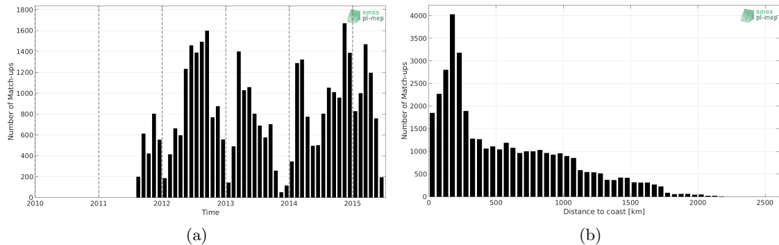
Figure 1: Number of match-ups between Sea mammals and Aquarius-L3-OR-V5-7DAY-RUNNING-RAIN-MASK-1DEG SSS as a function of time (a) and as function of the distance to coast (b) over the Global Ocean Pi-MEP region and for the full satellite product period.
