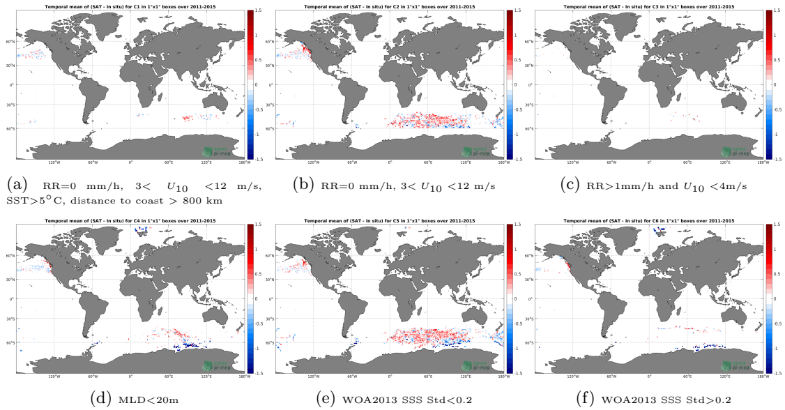
Figure 12: Temporal mean gridded over spatial boxes of size 1^\circ \times 1^\circ of \Delta SSS (Aquarius-L3-OR-V5-7DAY-RUNNING-RAIN-MASK-1DEG - Sea mammals) for 6 different subdatasets corresponding to:RR=0 mm/h, 3 < U_{10} < 12 m/s, SST > 5^\circ\text{C} , distance to coast > 800 km (a), RR=0 mm/h, 3 < U_{10} < 12 m/s (b), RR > 1 mm/h and U_{10} < 4 m/s (c),MLD < 20 m (d),WOA2013 SSS Std < 0.2 (e),WOA2013 SSS Std > 0.2 (f).
