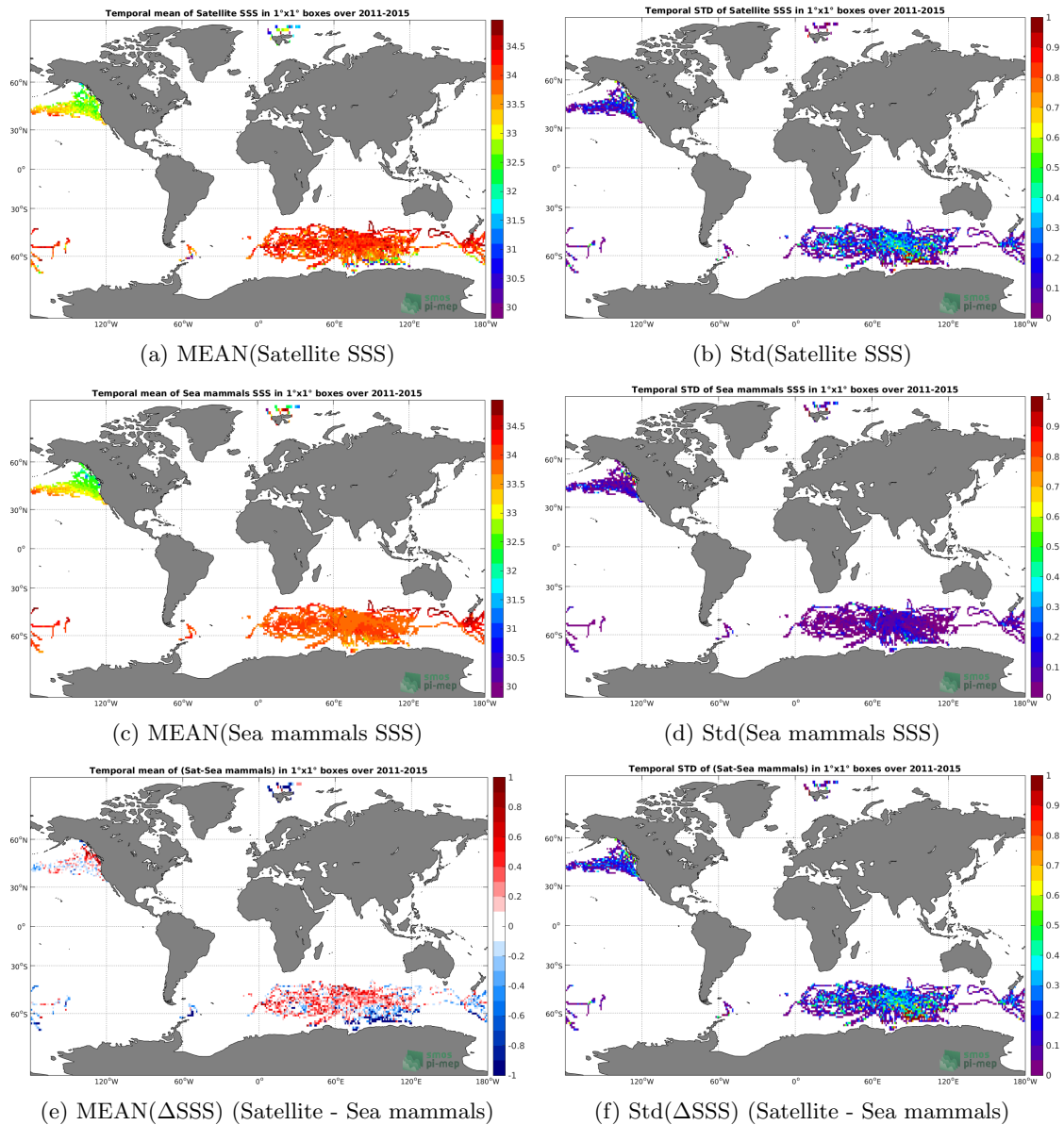
Figure 6: Temporal mean (left) and Std (right) of SSS from Aquarius-L3-OR-V5-7DAY-RUNNING-RAIN-MASK-1DEG (top), Sea mammals (middle), and of \Delta SSS (Satellite - Sea mammals). Only match-up pairs are used to generate these maps.
