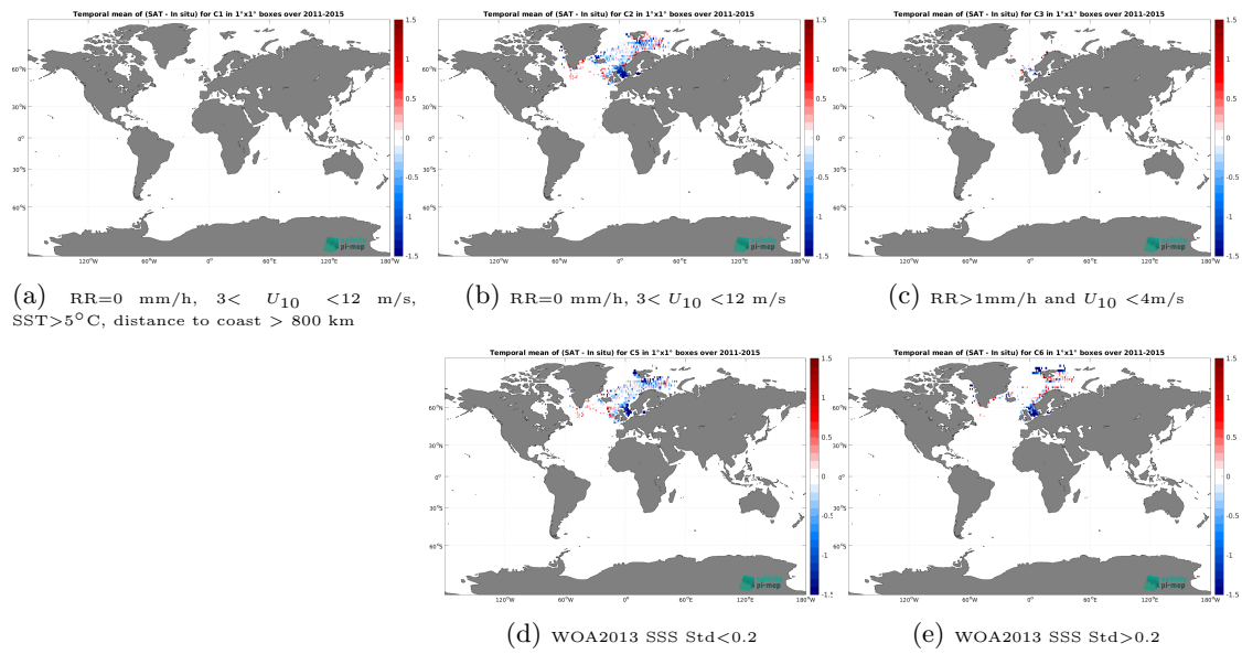
Figure 14: Temporal mean gridded over spatial boxes of size 1^\circ \times 1^\circ of \Delta SSS (Aquarius SSS L3 OR v5 - 7-Day running - Rain mask (NASA-GSFC) - ICES) for 5 different subdatasets corresponding to: RR=0 mm/h, 3 < U_{10} < 12 m/s, SST > 5^\circ\text{C} , distance to coast > 800 km (a), RR=0 mm/h, 3 < U_{10} < 12 m/s (b), RR > 1 mm/h and U_{10} < 4 m/s (c), WOA2013 SSS Std < 0.2 (d), WOA2013 SSS Std > 0.2 (e).
