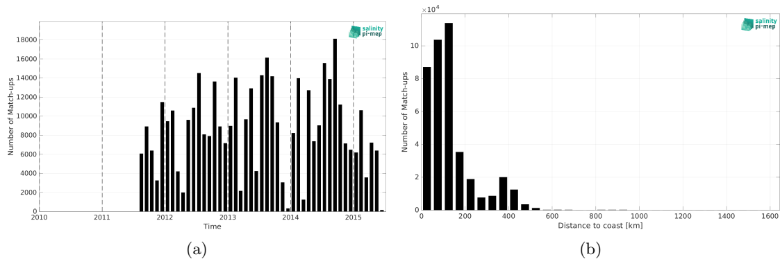
Figure 2: Number of match-ups between ICES and Aquarius SSS L3 OR v5 - 7-Day running - Rain mask (NASA-GSFC) SSS as a function of time (a) and as function of the distance to coast (b) over the Global Ocean Pi-MEP region and for the full satellite product period.
