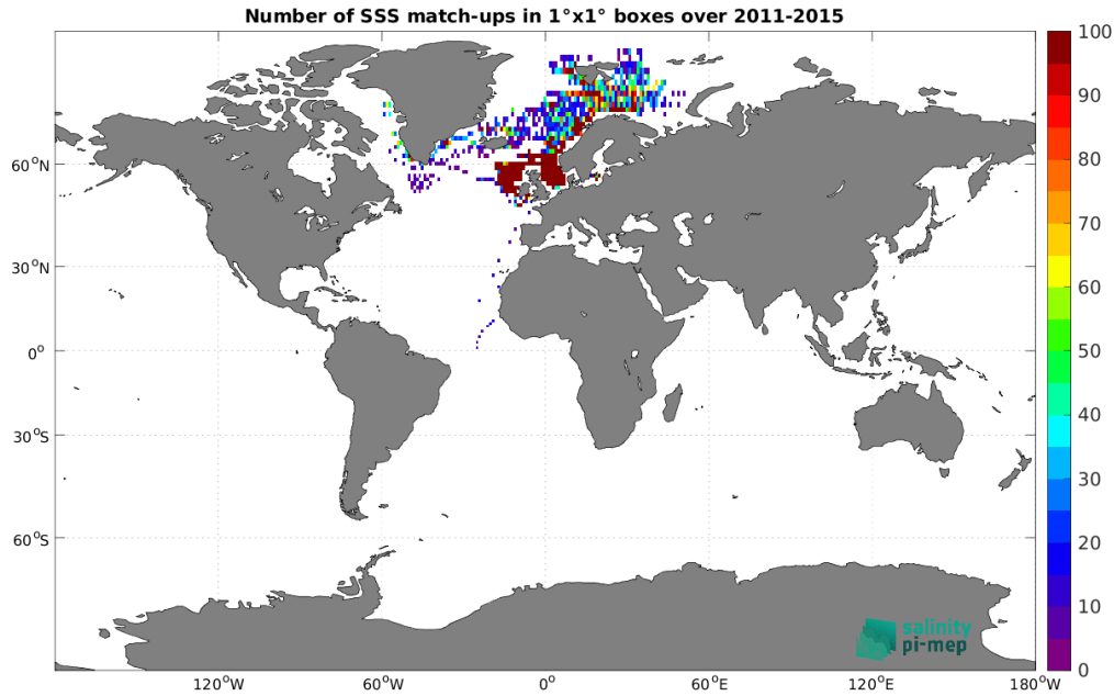
Figure 5: Number of SSS match-ups between ICES SSS and the Aquarius SSS L3 OR v5 - 7-Day running - Rain mask (NASA-GSFC) SSS product for the Global Ocean Pi-MEP region over 1^\circ \times 1^\circ boxes and for the full satellite product period.
