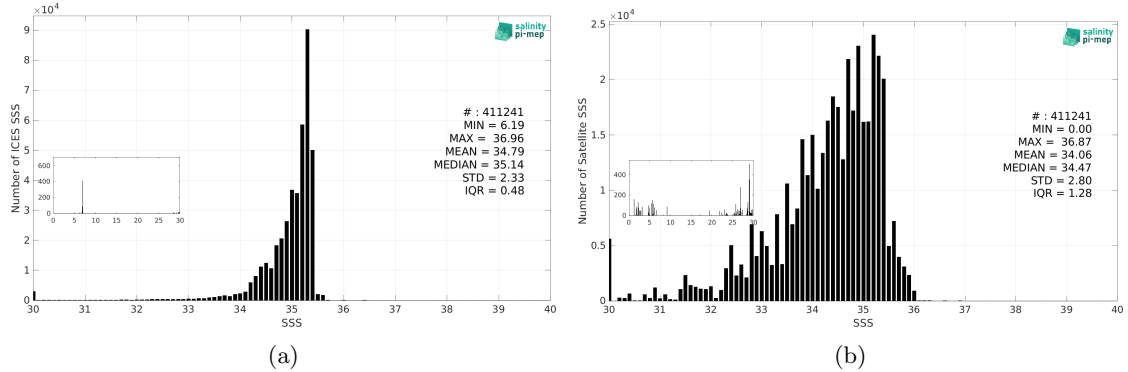
Figure 3: Histograms of SSS from ICES (a) and Aquarius SSS L3 OR v5 - 7-Day running - Rain mask (NASA-GSFC) (b) considering all match-up pairs per bins of 0.1 over the Global Ocean Pi-MEP region and for the full satellite product period.
