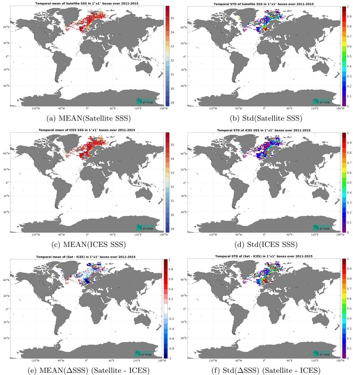
Figure 7: Temporal mean (left) and Std (right) of SSS from Aquarius SSS L3 OR v5 - 7-Day running - Rain mask (NASA-GSFC) (top), ICES (middle), and of \Delta SSS (Satellite - ICES). Only match-up pairs are used to generate these maps.
