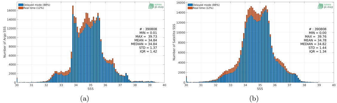
Figure 2: Histograms of SSS from Argo (a) and Aquarius SSS L3 OR v5 - 7-Day running - Rain mask (NASA-GSFC) (b) considering all match-up pairs per bins of 0.1 over the Global Ocean Pi-MEP region and for the full satellite product period.
