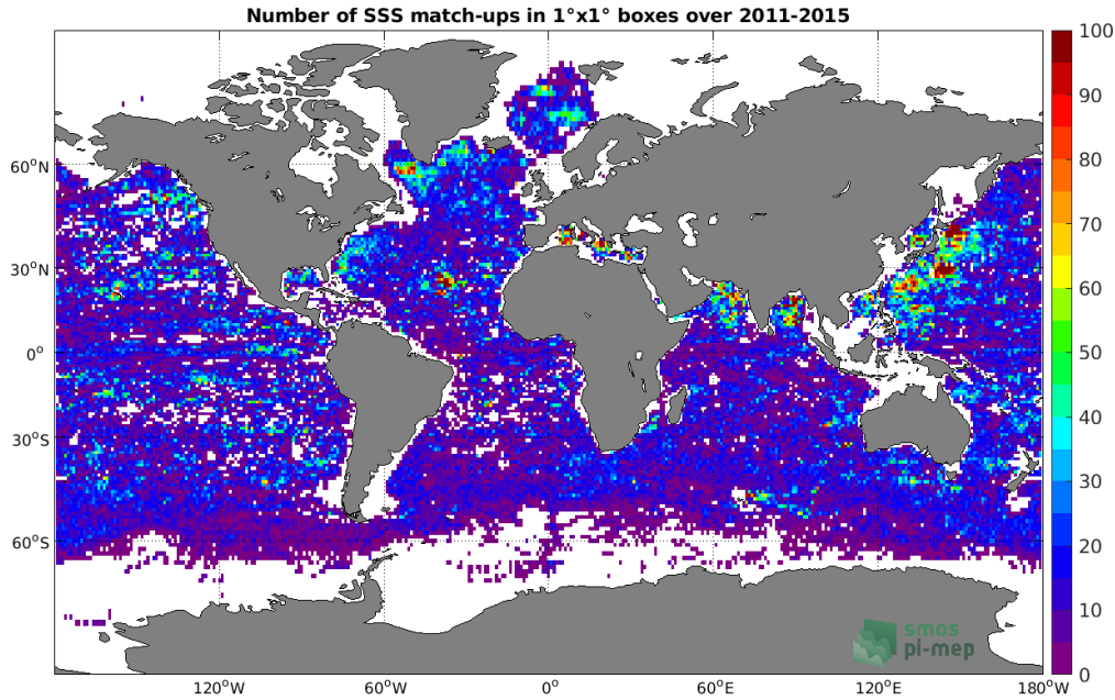
Figure 4: Number of SSS match-ups between Argo SSS and the Aquarius SSS L3 OR v5 - 7-Day running - Rain mask (NASA-GSFC) SSS product for the Global Ocean Pi-MEP region over 1^{\circ} \times 1^{\circ} boxes and for the full satellite product period.
