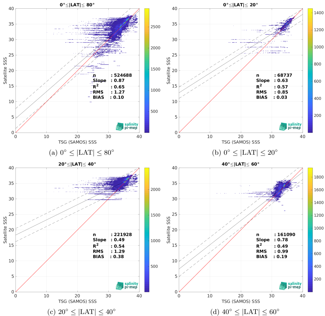
Figure 10: Contour maps of the concentration of Aquarius SSS L3 OR v5 - Monthly (NASA-GSFC) SSS (y-axis) versus TSG (SAMOS) SSS (x-axis) at match-up pairs for different latitude bands. For each plot, the red line shows x=y . The black thin and dashed lines indicate a linear fit through the data cloud and the \pm 95\% confidence levels, respectively. The number match-up pairs n , the slope and R^2 coefficient of the linear fit, the root mean square (RMS) and the mean bias between satellite and in situ data are indicated for each latitude band in each plot.
