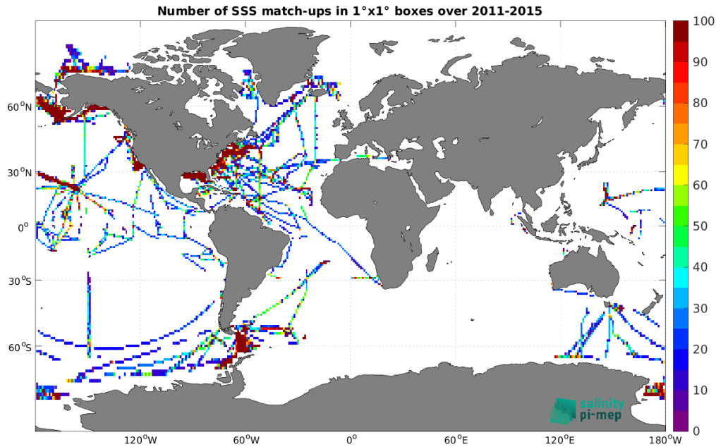
Figure 5: Number of SSS match-ups between TSG (SAMOS) SSS and the Aquarius SSS L3 OR v5 - Monthly (NASA-GSFC) SSS product for the Global Ocean Pi-MEP region over 1^\circ \times 1^\circ boxes and for the full satellite product period.
