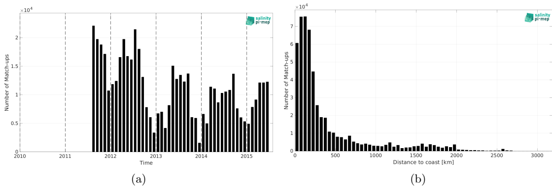
Figure 2: Number of match-ups between TSG (SAMOS) and Aquarius SSS L3 OR v5 - Monthly (NASA-GSFC) SSS as a function of time (a) and as function of the distance to coast (b) over the Global Ocean Pi-MEP region and for the full satellite product period.
