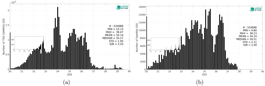
Figure 3: Histograms of SSS from TSG (SAMOS) (a) and Aquarius SSS L3 OR v5 - Monthly (NASA-GSFC) (b) considering all match-up pairs per bins of 0.1 over the Global Ocean Pi-MEP region and for the full satellite product period.
