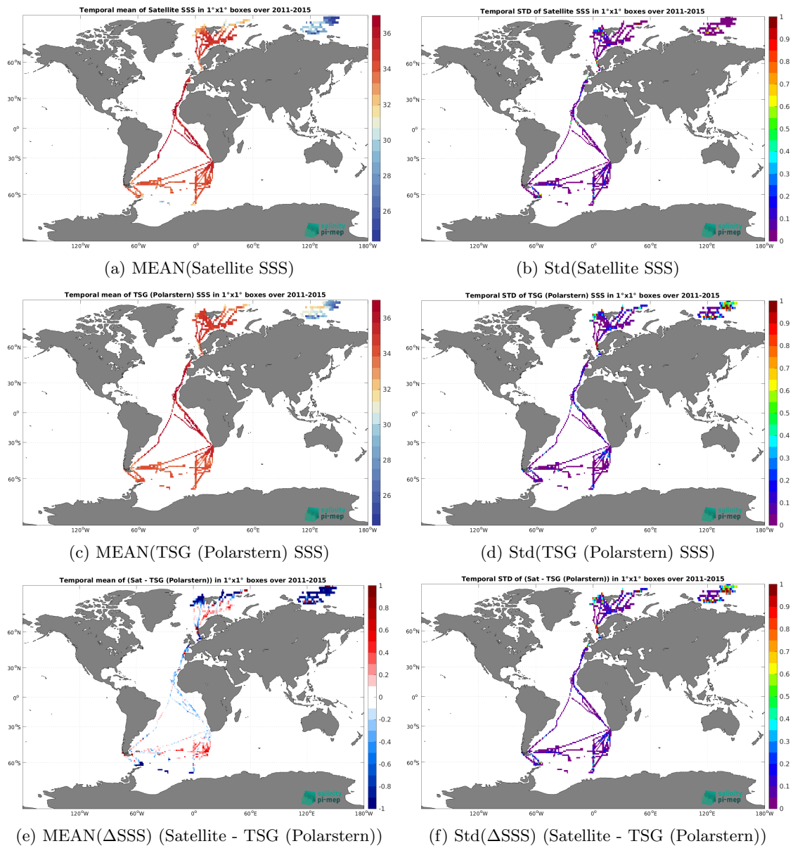
Figure 7: Temporal mean (left) and Std (right) of SSS from Aquarius SSS L3 OR v5 - Monthly (NASA-GSFC) (top), TSG (Polarstern) (middle), and of \Delta SSS (Satellite - TSG (Polarstern)). Only match-up pairs are used to generate these maps.
