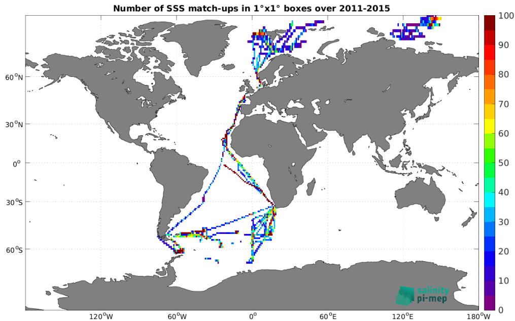
Figure 5: Number of SSS match-ups between TSG (Polarstern) SSS and the Aquarius SSS L3 OR v5 - Monthly (NASA-GSFC) SSS product for the Global Ocean Pi-MEP region over 1^\circ \times 1^\circ boxes and for the full satellite product period.
