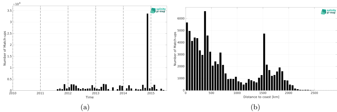
Figure 2: Number of match-ups between TSG (Polarstern) and Aquarius SSS L3 OR v5 - Monthly (NASA-GSFC) SSS as a function of time (a) and as function of the distance to coast (b) over the Global Ocean Pi-MEP region and for the full satellite product period.
