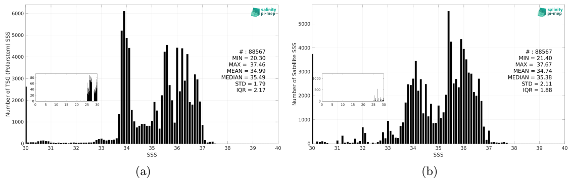
Figure 3: Histograms of SSS from TSG (Polarstern) (a) and Aquarius SSS L3 OR v5 - Monthly (NASA-GSFC) (b) considering all match-up pairs per bins of 0.1 over the Global Ocean Pi-MEP region and for the full satellite product period.
