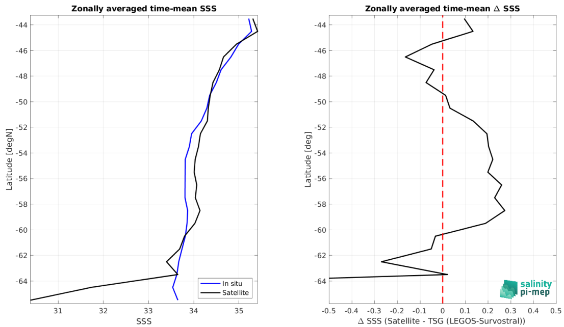
Figure 9: Left panel: Zonal mean SSS from Aquarius SSS L3 OR v5 - Monthly (NASA-GSFC) satellite product (black) and from TSG (LEGOS-Survostral) (blue). Right panel: Zonal mean of \Delta SSS (Satellite - TSG (LEGOS-Survostral)) for all the collected Pi-MEP match-up pairs estimated over the full satellite product period.
