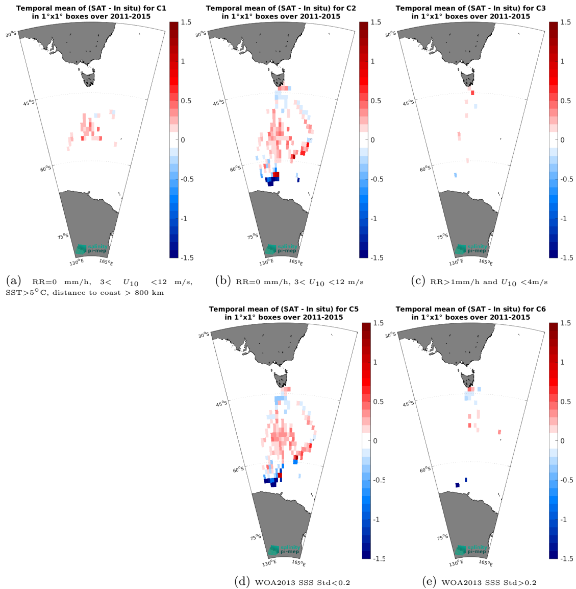
Figure 14: Temporal mean gridded over spatial boxes of size 1^\circ \times 1^\circ of \Delta SSS (Aquarius SSS L3 OR v5 - Monthly (NASA-GSFC) - TSG (LEGOS-Survostral)) for 5 different subdatasets corresponding to:RR=0 mm/h, 3 < U_{10} < 12 m/s, SST>5°C, distance to coast > 800 km (a), RR=0 mm/h, 3 < U_{10} < 12 m/s (b), RR>1mm/h and U_{10} < 4 m/s (c), WOA2013 SSS Std<0.2 (d), WOA2013 SSS Std>0.2 (e).
