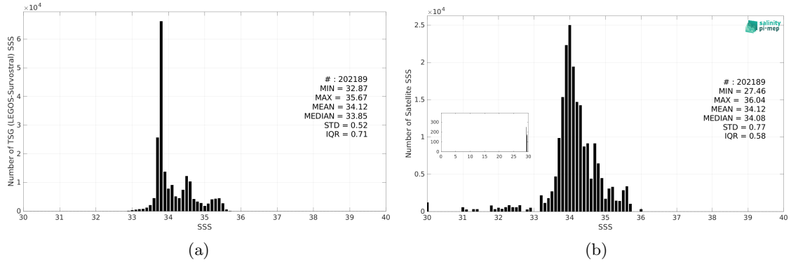
Figure 3: Histograms of SSS from TSG (LEGOS-Survostral) (a) and Aquarius SSS L3 OR v5 - Monthly (NASA-GSFC) (b) considering all match-up pairs per bins of 0.1 over the Global Ocean Pi-MEP region and for the full satellite product period.
