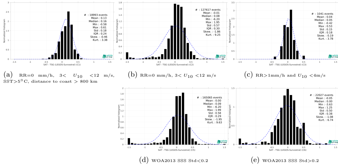
Figure 15: Normalized histogram of \Delta SSS (Aquarius SSS L3 OR v5 - Monthly (NASA-GSFC) - TSG (LEGOS-Survostral)) for 5 different subdatasets corresponding to: RR=0 mm/h, 3 < U_{10} < 12 m/s, SST>5°C, distance to coast > 800 km (a), RR=0 mm/h, 3 < U_{10} < 12 m/s (b), RR>1mm/h and U_{10} < 4 m/s (c), WOA2013 SSS Std<0.2 (d), WOA2013 SSS Std>0.2 (e).
