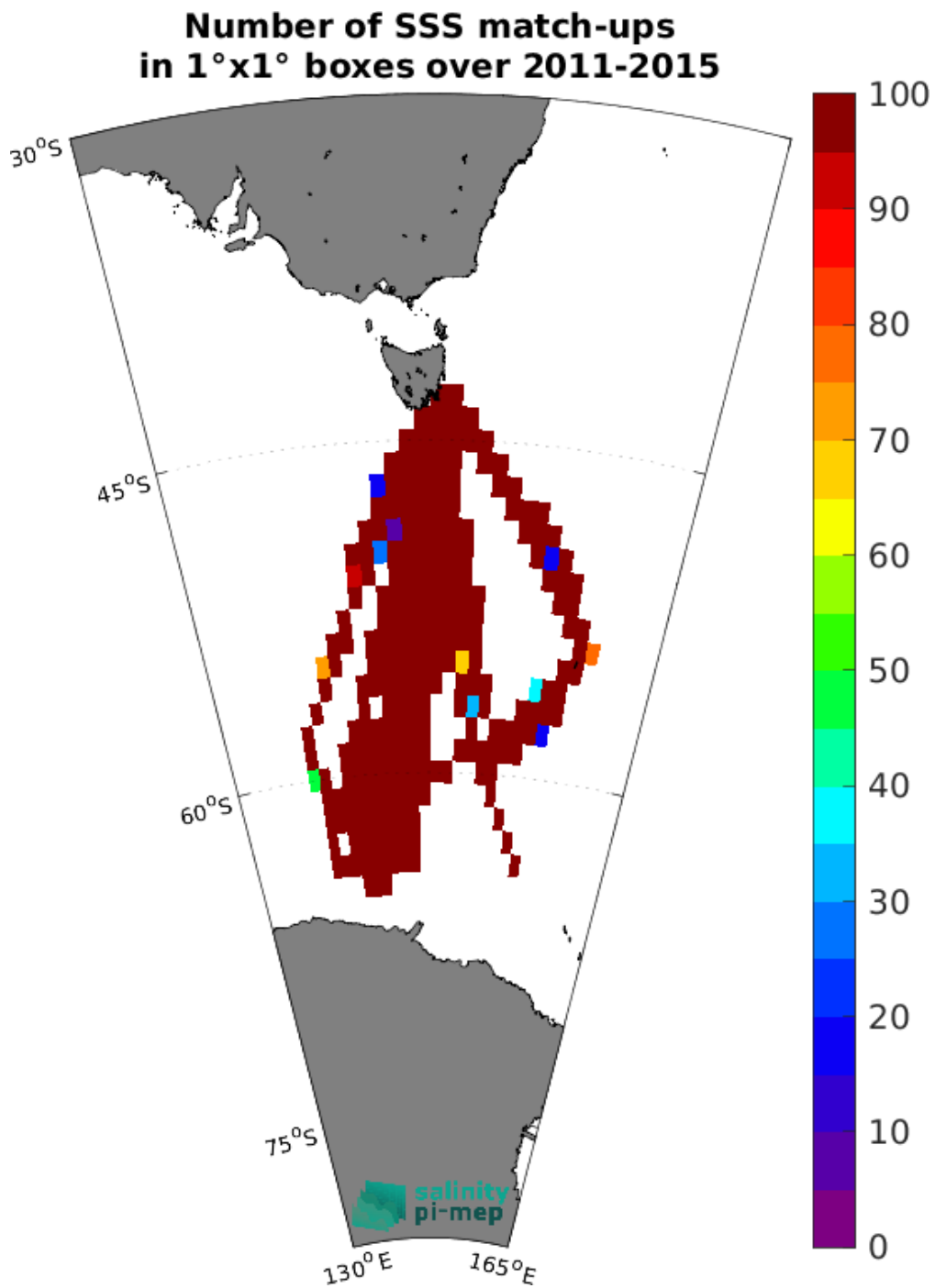
Figure 5: Number of SSS match-ups between TSG (LEGOS-Survostral) SSS and the Aquarius SSS L3 OR v5 - Monthly (NASA-GSFC) SSS product for the Global Ocean Pi-MEP region over 1^\circ \times 1^\circ boxes and for the full satellite product period.
