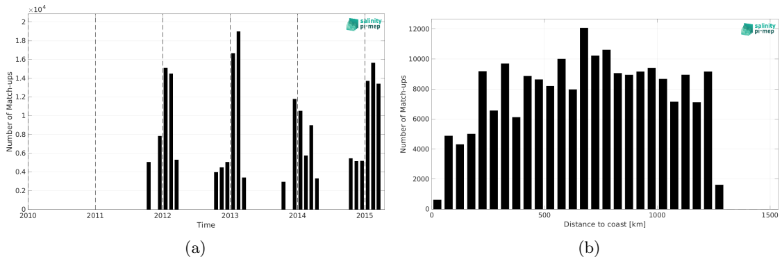
Figure 2: Number of match-ups between TSG (LEGOS-Survostral) and Aquarius SSS L3 OR v5 - Monthly (NASA-GSFC) SSS as a function of time (a) and as function of the distance to coast (b) over the Global Ocean Pi-MEP region and for the full satellite product period.
