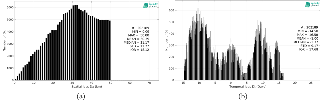
Figure 6: Histograms of the spatial (a) and temporal (b) lags between the location/time of the TSG (LEGOS-Survostral) measurement and the date of the corresponding Aquarius SSS L3 OR v5 - Monthly (NASA-GSFC) SSS pixel.
