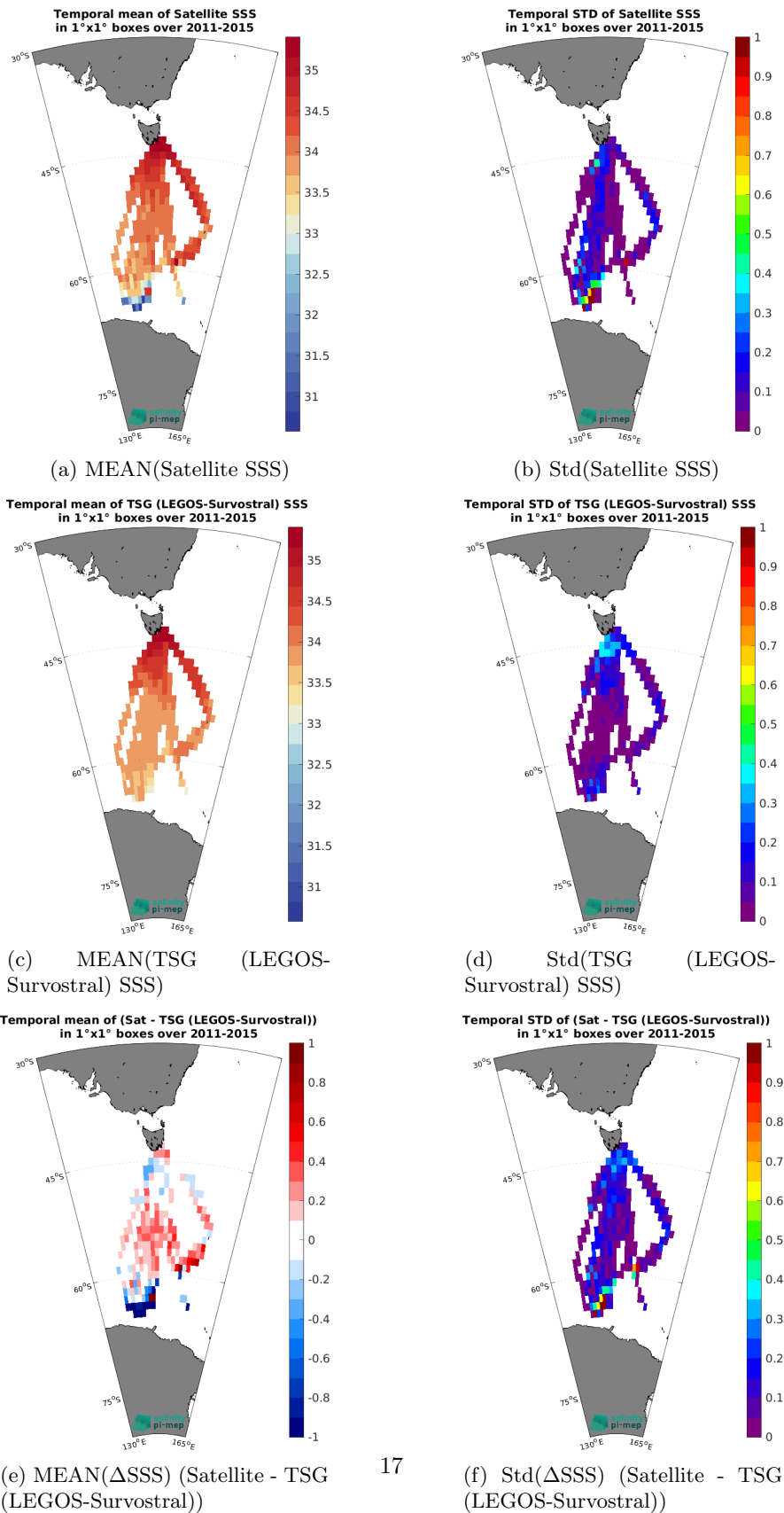
Figure 6: Temporal mean (left) and Std (right) of SSS from Aquarius SSS L3 OR v5 - Monthly (NASA-GSFC) (top), TSG (LEGOS-Survostral) (middle), and of \Delta SSS (Satellite - TSG (LEGOS-Survostral)). Only match-up pairs are used to generate these maps.
