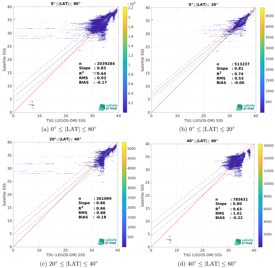
Figure 9: Contour maps of the concentration of Aquarius SSS L3 OR v5 - Monthly (NASA-GSFC) SSS (y-axis) versus TSG (LEGOS-DM) SSS (x-axis) at match-up pairs for different latitude bands. For each plot, the red line shows x=y . The black thin and dashed lines indicate a linear fit through the data cloud and the \pm 95\% confidence levels, respectively. The number of match-up pairs n , the slope and R^2 coefficient of the linear fit, the root mean square (RMS) and the mean bias between satellite and in situ data are indicated for each latitude band in each plot.
