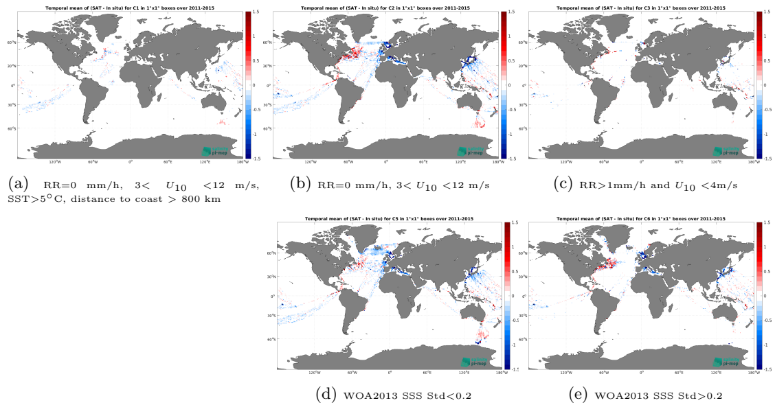
Figure 12: Temporal mean gridded over spatial boxes of size 1^\circ \times 1^\circ of \Delta SSS (Aquarius SSS L3 OR v5 - Monthly (NASA-GSFC) - TSG (LEGOS-DM)) for 5 different subdatasets corresponding to: RR=0 mm/h, 3 < U_{10} < 12 m/s, SST > 5^\circ\text{C} , distance to coast > 800 km (a), RR=0 mm/h, 3 < U_{10} < 12 m/s (b), RR > 1 mm/h and U_{10} < 4 m/s (c), WOA2013 SSS Std < 0.2 (d), WOA2013 SSS Std > 0.2 (e).
