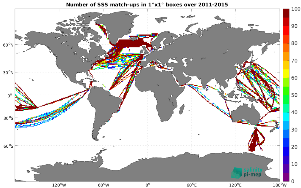
Figure 4: Number of SSS match-ups between TSG (LEGOS-DM) SSS and the Aquarius SSS L3 OR v5 - Monthly (NASA-GSFC) SSS product for the Global Ocean Pi-MEP region over 1^\circ \times 1^\circ boxes and for the full satellite product period.
